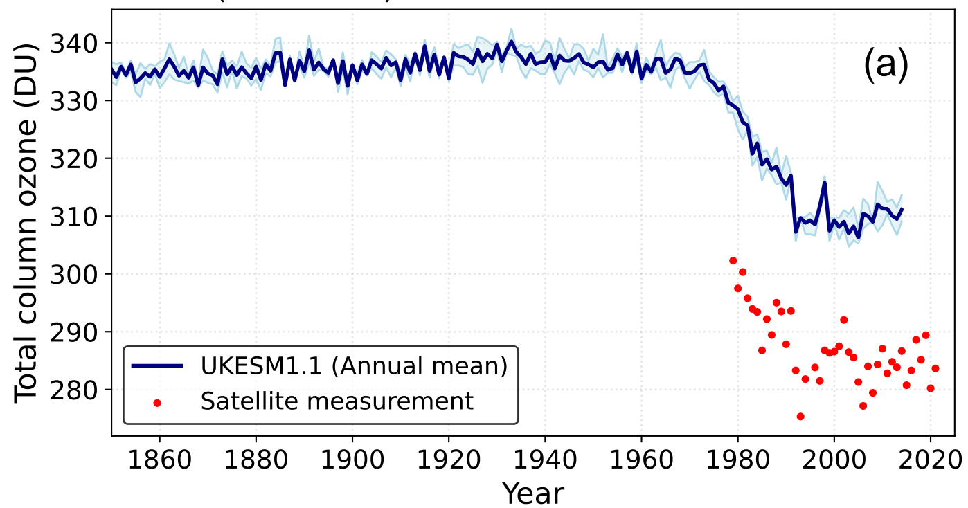
Antarctica (90°S-60°S)
