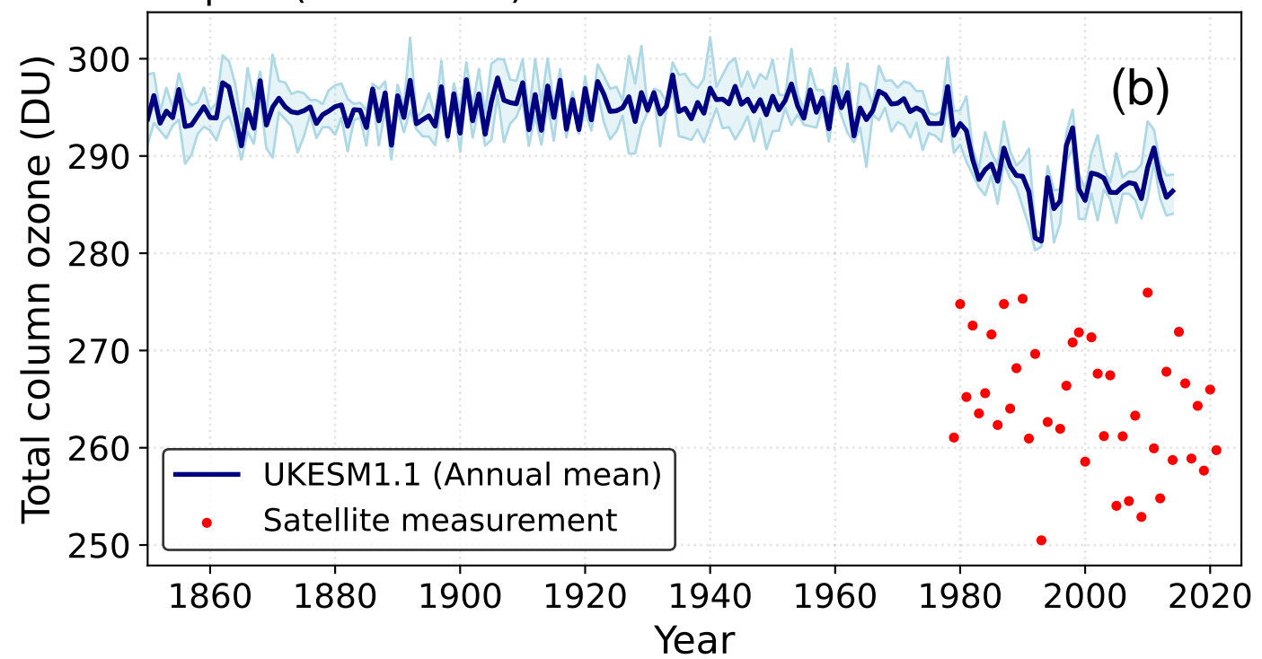
Arctic (60°N-90°N)
