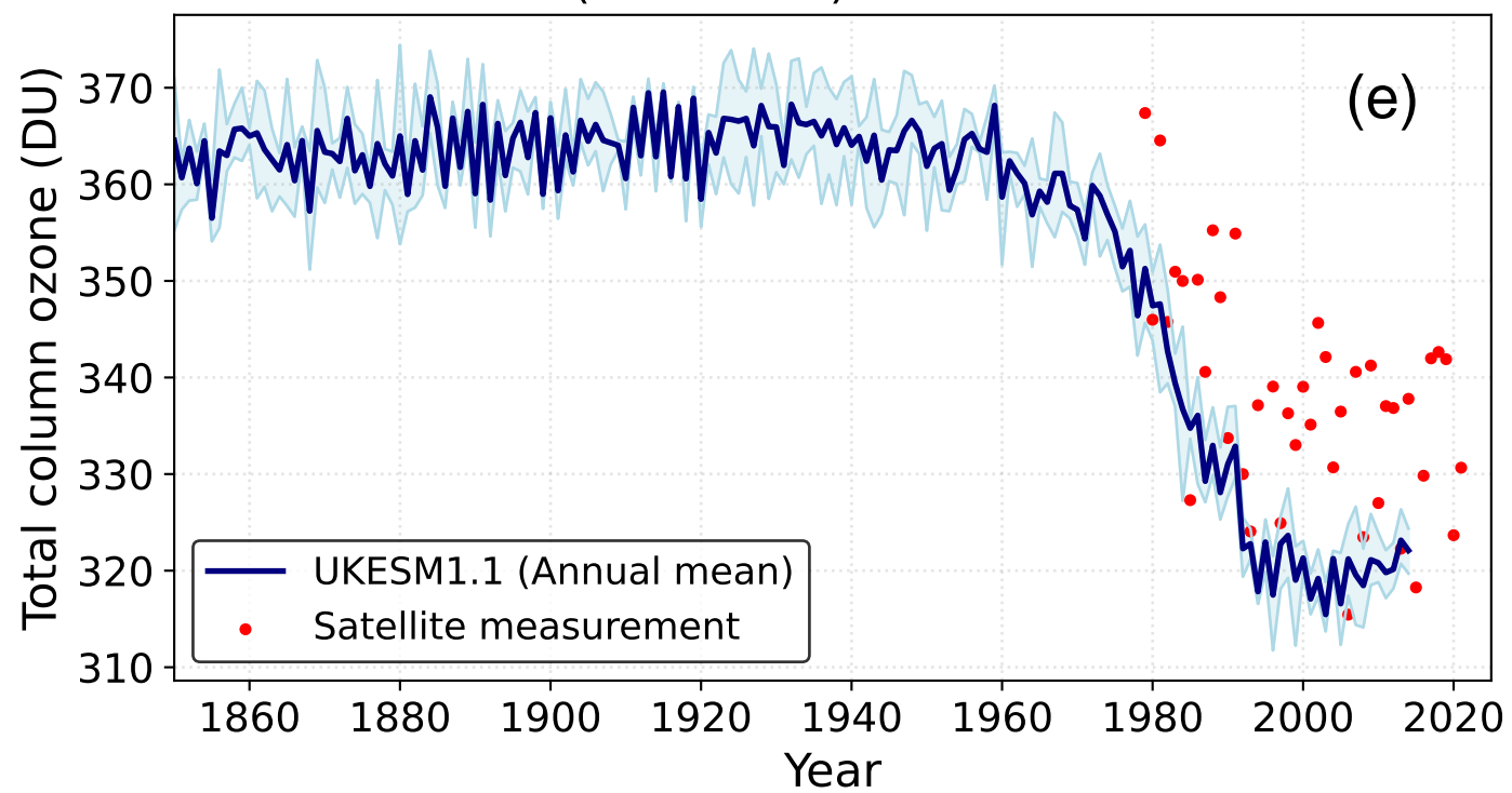
SH mid-latitudes (60°S-30°S)
