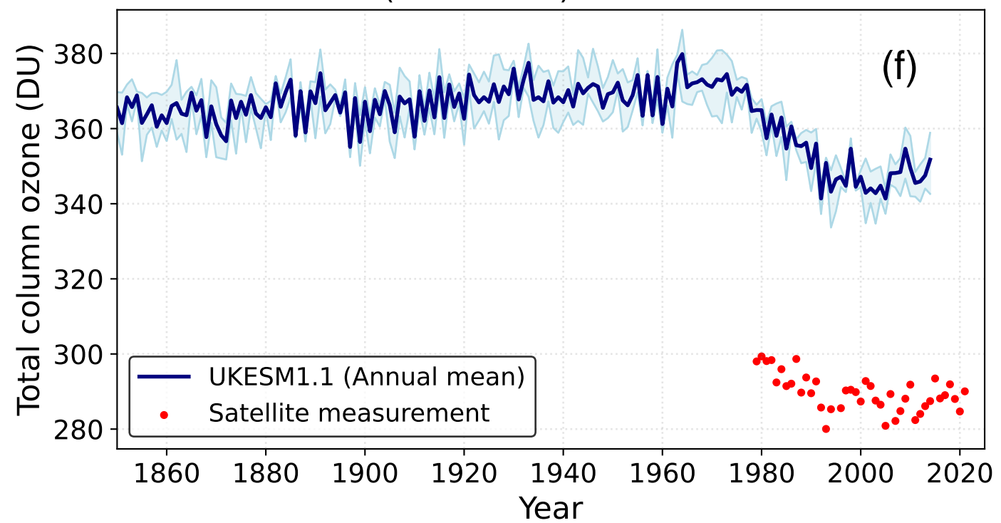
NH mid-latitudes (30°N-60°N)
