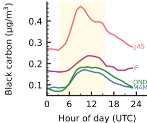
(e) Black carbon
