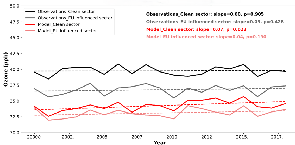
Figure S7. Yearly trend average of observed O 3 (black) and Model O 3 (red) at Mace head, separated into clean sector and EU-influenced sector.
