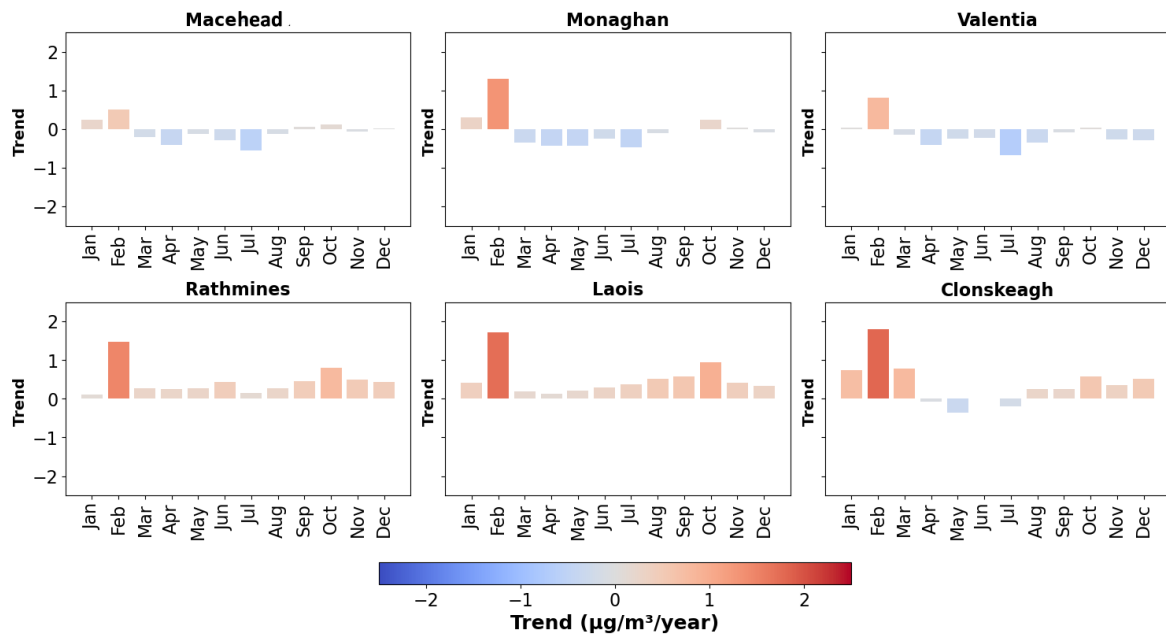
Figure S2. Monthly trend analysis of O 3 at different sites for 15 years period.
