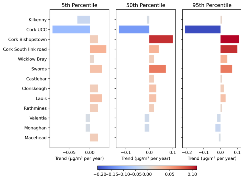
Figure S3. Trend in O 3 Percentiles observed at different stations.
