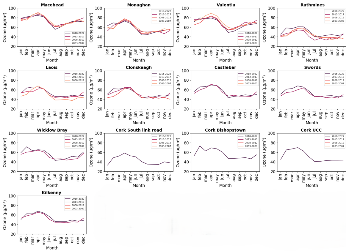
Figure S1. Five-year monthly variation in O 3 concentration at different sites in Ireland.
