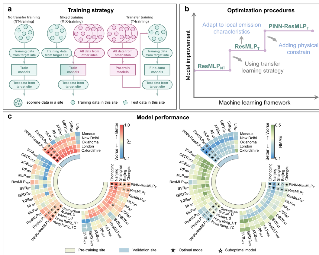
Figure 2. Schematic of the machine learning framework for predicting isoprene concentration. (a) A sketch of the training strategy. (b) The improvement of the machine learning framework. (c) Comparisons of statistical performance across different algorithms in individual sites. RF, XGB, GBDT, SVM, and LR represent Random Forest, eXtreme Gradient Boosting, Gradient Boosting Decision Tree, Support Vector Machine, and Linear Regression, respectively.
