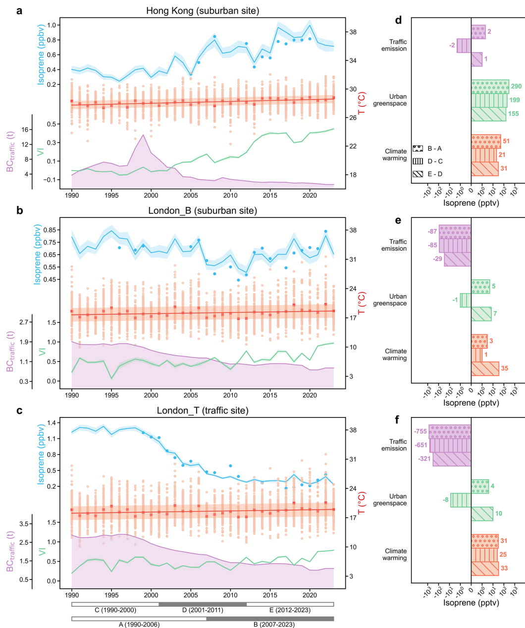
Figure 4. Long-term trends of the summertime isoprene and the drivers. (a–c) Variations of isoprene concentrations (blue lines for simulated, blue dots for observed), temperature ( T ), urban greenspace (VI) and traffic emissions ( \text{BC}_{\text{traffic}} ) in Hong Kong (a) and London (b, c) . The red dots and red line represent temperature and the fitted trend for the mean temperature, respectively. The bands represent 95 % confidence intervals. (d–f) Changes in isoprene concentrations caused by climate warming, urban greenspace and traffic emissions in Hong Kong (d) and London (e, f) during different periods.
