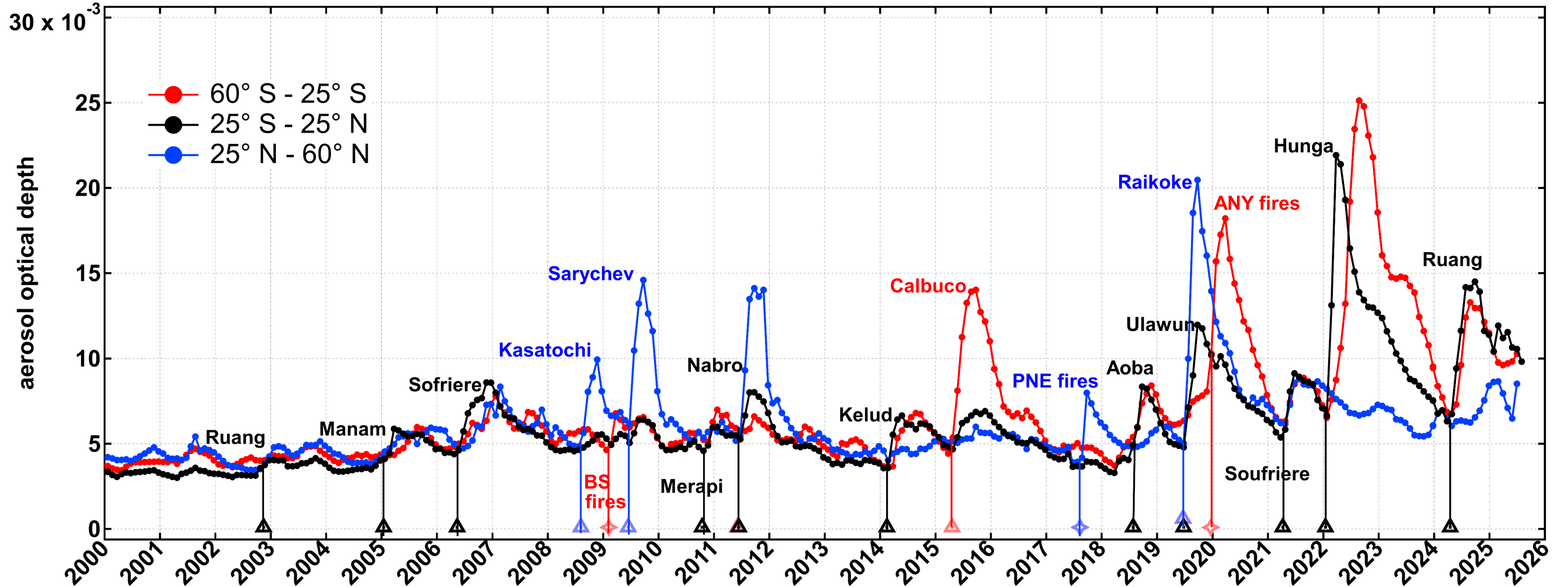
GloSSAC+SAGE III stratospheric AOD@525 nm above 380 K
