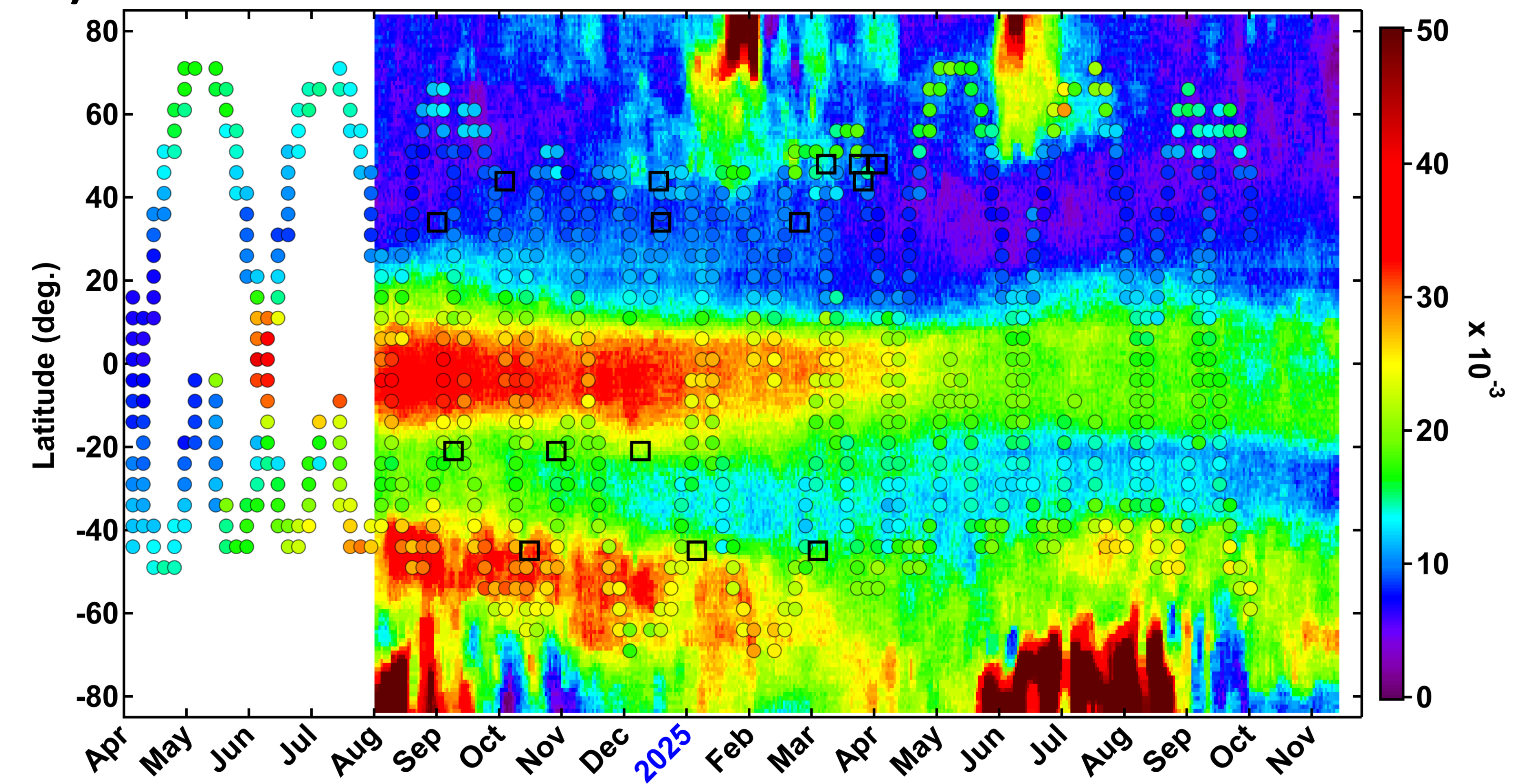
b) EarthCARE/ATLID L1 and ISS/SAGE III, sAOD 355 nm non-attenuated
