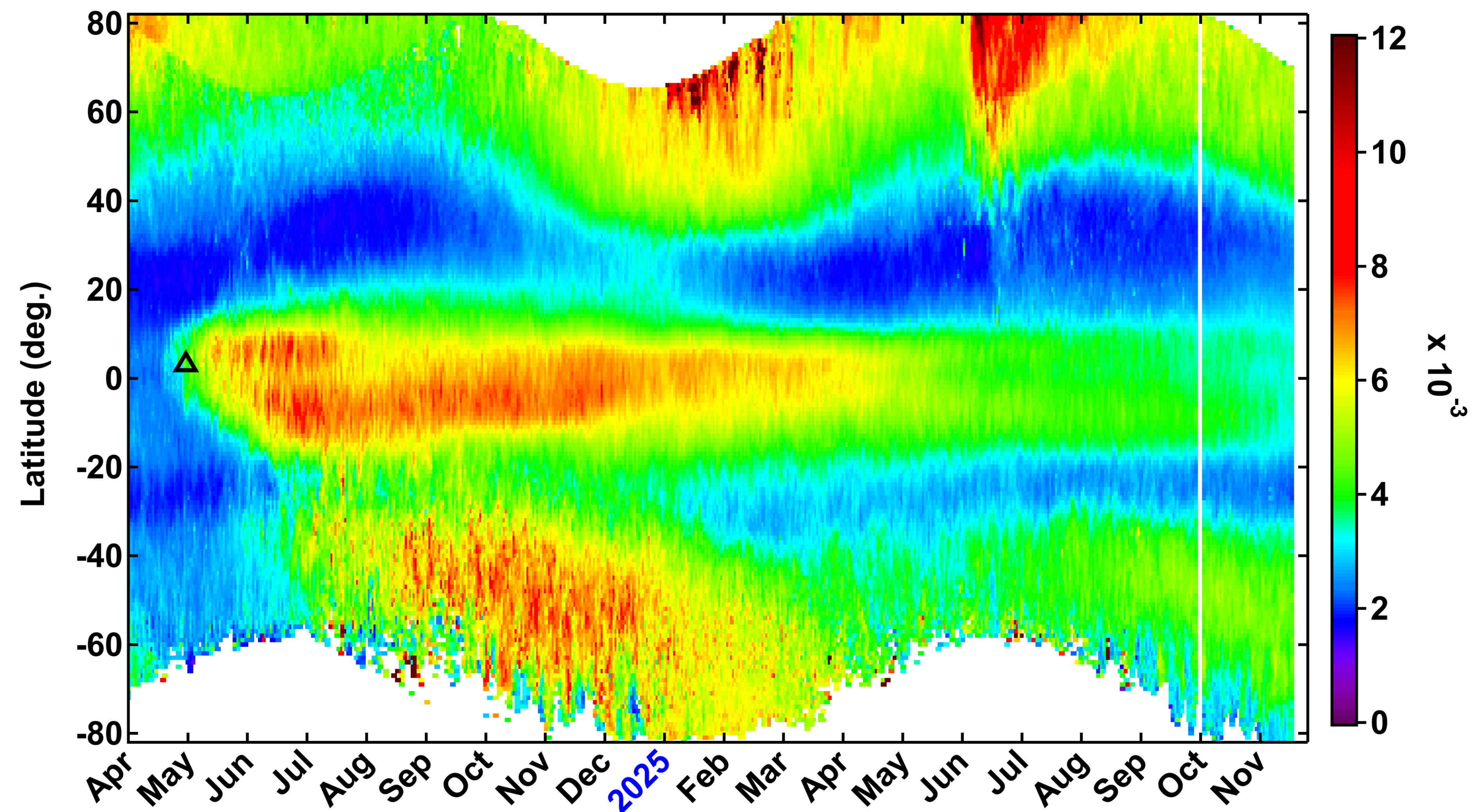
a) NOAA-21/OMPS-LP and ISS/SAGE III, sAOD 869 nm
