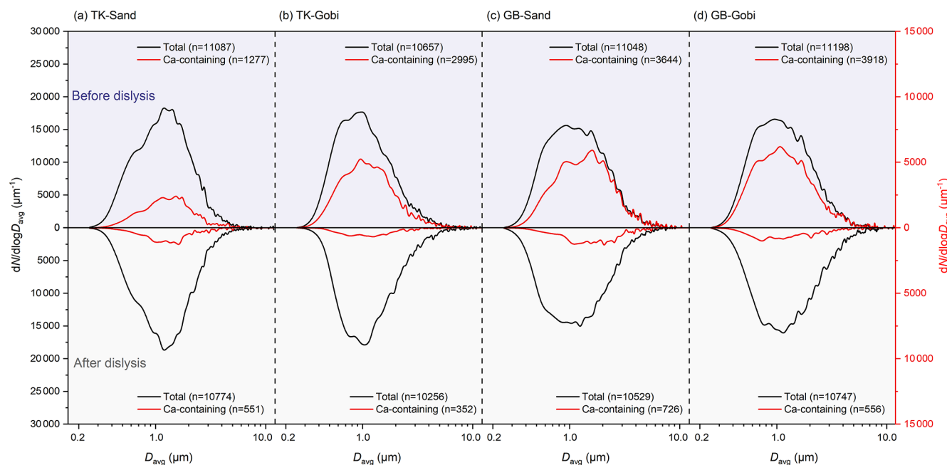
Figure 3. Particle number size distributions of Ca-containing and total dust particles generated from sandy (Sand) and gravel (Gobi) surface soils of the Taklimakan (TK) and Gobi (GB) Desert.
