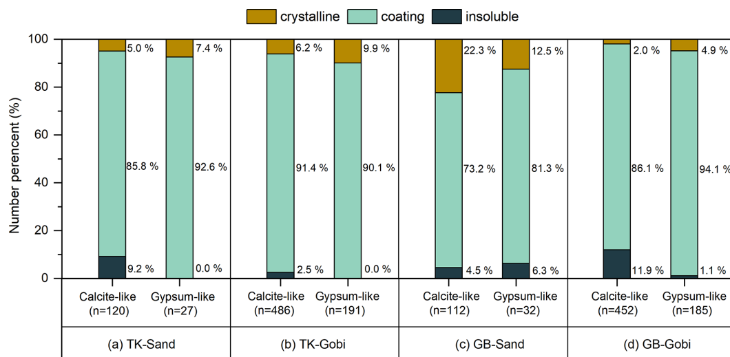
Figure 5. Relative particle number percentage of Ca-O-rich (calcite-like) and Ca-S-containing (gypsum-like) particles in different mixing states. The numbers in the parentheses are the counts of detected Ca-O-rich and Ca-S-containing particles.
