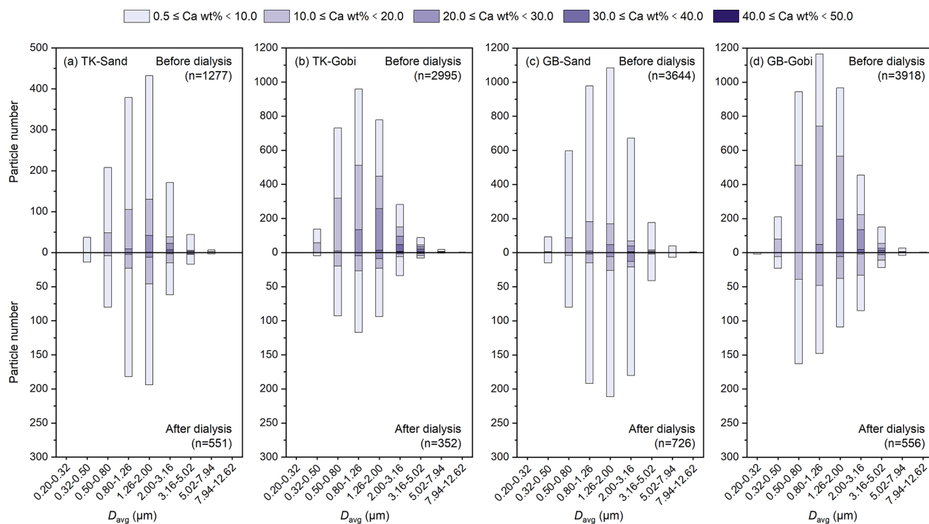
Figure 2. Relationship between particle size ( \mu\text{m} ) and calcium content (relative weight percentage in single particle, Ca wt %) for Ca-bearing particles before and after water dialysis.
