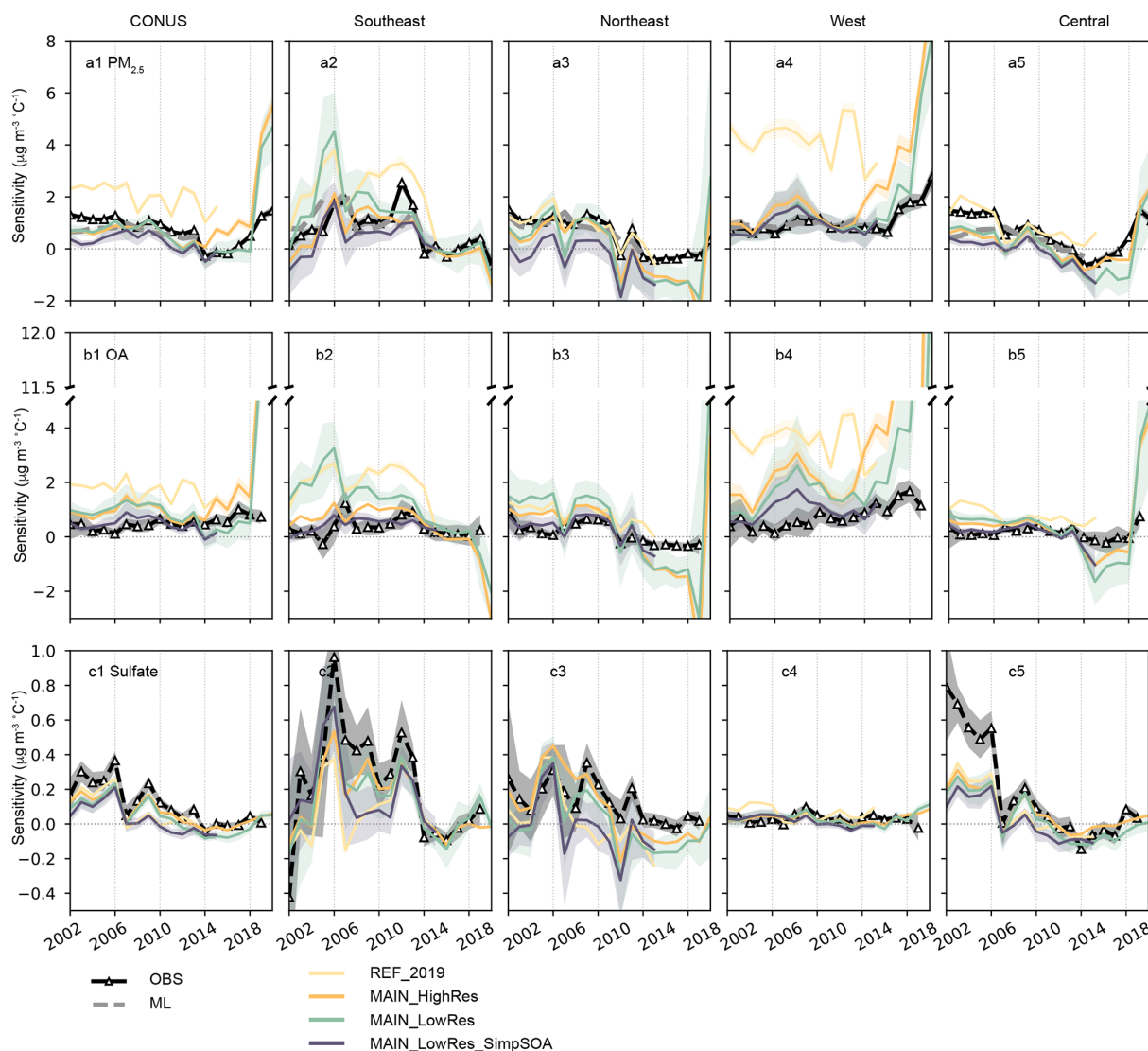
Figure 2. Regional-aggregated temperature sensitivity of PM 2.5 , organic aerosols (OA), and sulfate for 5-year running time windows, derived from ground-based observations, machine-learning-modeled data (2000–2016), and four GEOS-Chem simulation cases. The shaded areas represent the 95 % confidence interval across each region. Panels (a1)–(a5) show the PM 2.5 sensitivity for the contiguous US (a1), the Southeast US (a2), the Northeast US (a3), the West US (a4), and the Central US (a5); (b1)–(b5) show the OA sensitivity for each region; (c1)–(c5) show the sulfate sensitivity for each region.
