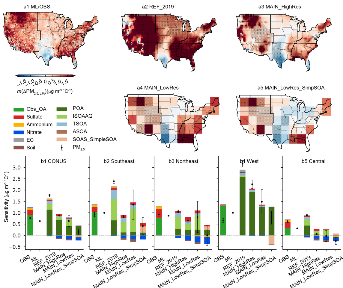
Figure 1. Spatial distribution and regionally aggregated temperature sensitivity of summertime PM 2.5 and its major components during 2000–2016, derived from ground-based observations, machine-learning (ML) modeled datasets, and GEOS-Chem simulations. Maps show the spatial distribution of PM 2.5 temperature sensitivity derived from ML-modeled data and observations (a1), GEOS-Chem REF_2019 case simulations (a2), MAIN_HighRes case simulations (a3), MAIN_LowRes case (a4), and MAIN_LowRes_SimpSOA case (a5). Triangle markers represent fitted sensitivities from observations with p -value < 0.05. Stippling represents fitted temperature sensitivities with p -value < 0.05 in GEOS-Chem. Bar charts show regionally aggregated temperature sensitivities for PM 2.5 and its major components across the contiguous United States (b1), the Southeastern US (b2), the Northeastern US (b3), the Western US (b4), and the Central US (b5).
