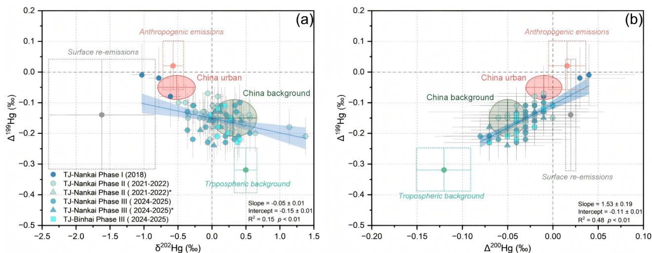
Figure 3. Phase variations of Hg isotopic compositions in Tianjin. (a) \delta^{202}\text{Hg} versus \Delta^{199}\text{Hg} , (b) \Delta^{200}\text{Hg} versus \Delta^{199}\text{Hg} of GEM in the TJ-Nankai (urban) and TJ-Binhai (suburban) sites. The corrected \delta^{202}\text{Hg} values for passive MerPAS samples are marked with an asterisk ( \delta^{202}\text{Hg}^* ). Error bars of individual GEM samples indicate the 2\sigma analytical uncertainty. Light red, grey, and green rectangles represent the mean \pm 1 SD ranges of the estimated end-member isotopic compositions: anthropogenic GEM emissions (Wu et al., 2023), surface GEM re-emissions (Zhu et al., 2022; Fu et al., 2026), and tropospheric background GEM (Tang et al., 2024). Deep red and green ellipses represent the mean \pm 1 SD ranges of the compiled China urban and regional background GEM isotopic compositions (Zhang and Sun, 2026).
