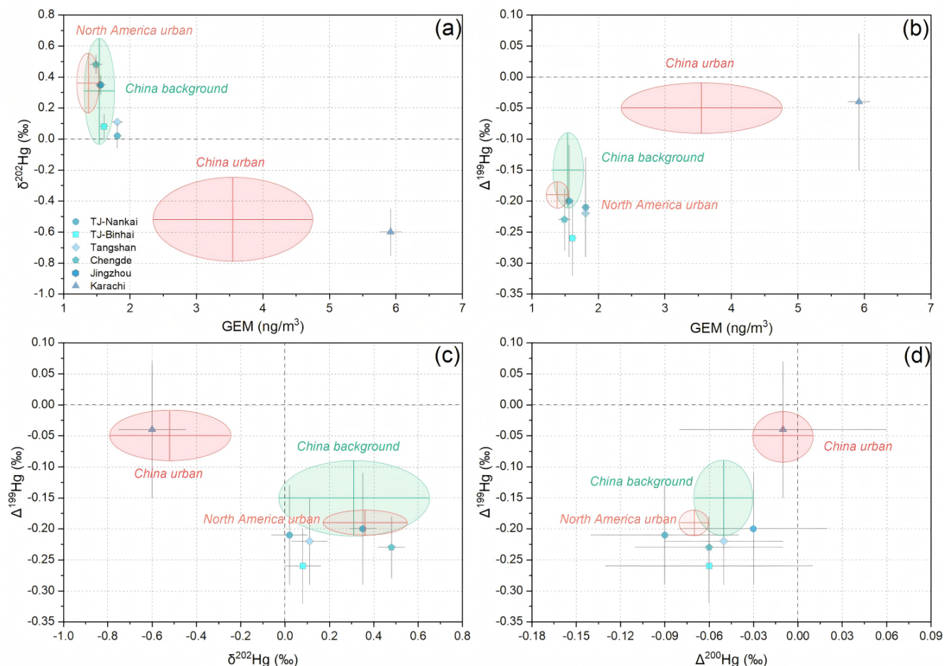
Figure 5. Regional comparison of GEM concentrations and isotopic compositions. (a) Concentrations versus \delta^{202}\text{Hg} , (b) concentrations versus \Delta^{199}\text{Hg} , (c) \delta^{202}\text{Hg} versus \Delta^{199}\text{Hg} , (d) \Delta^{200}\text{Hg} versus \Delta^{199}\text{Hg} of GEM across different sites. Error bars of individual GEM samples indicate the combined uncertainty calculated from the 2\sigma analytical uncertainty and the 2 SD of concurrently deployed paired MerPAS units. Deep red and green ellipses represent mean \pm 1 SD ranges of compiled urban and regional background GEM isotopic compositions in China (Zhang and Sun, 2026). Light red ellipse represents the mean \pm 1 SD range of the compiled urban GEM isotopic compositions in North America (Tate et al., 2023).
