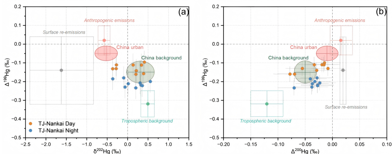
Figure 4. Diurnal variations in GEM isotopic compositions. (a) \delta^{202}\text{Hg} versus \Delta^{199}\text{Hg} , (b) \Delta^{200}\text{Hg} versus \Delta^{199}\text{Hg} of GEM in the TJ-Nankai (urban) site. Error bars of individual GEM samples indicate the 2\sigma analytical uncertainty. Light red, grey, and green rectangles represent the mean \pm 1 SD ranges of the estimated end-member isotopic compositions: anthropogenic GEM emissions (Wu et al., 2023), surface GEM re-emissions (urban soil and marine re-emissions) (Zhu et al., 2022; Fu et al., 2026), and tropospheric background GEM (Tang et al., 2024). Deep red and green ellipses represent the mean \pm 1 SD ranges of the compiled China urban and regional background GEM isotopic compositions (Zhang and Sun, 2026).
