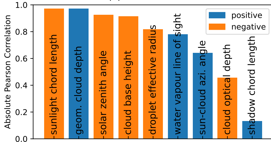
(a) Correlation to \varepsilon
