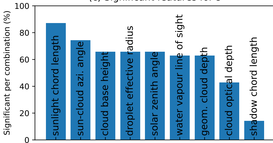
(c) Significant features for \varepsilon
