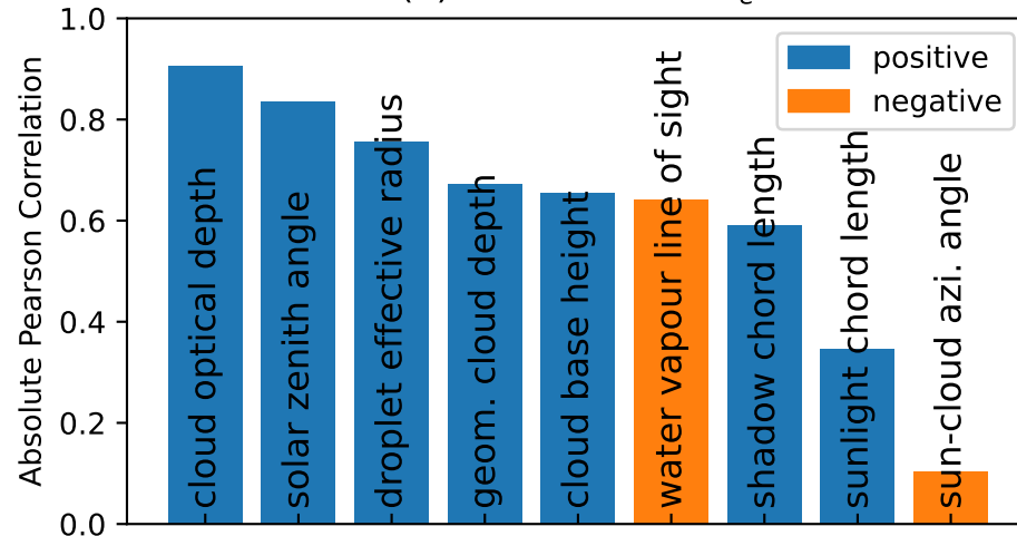
(b) Correlation to x_e
