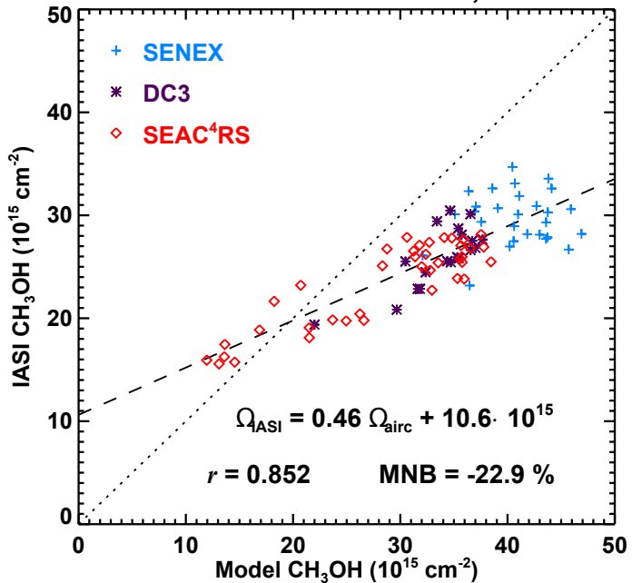
b. IASI and model columns, with AKs
