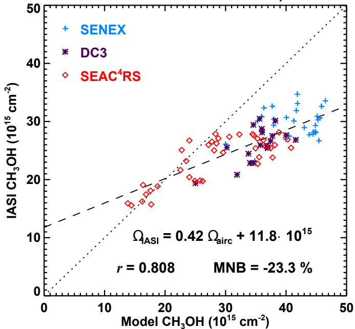
a. IASI and model columns, no AKs
