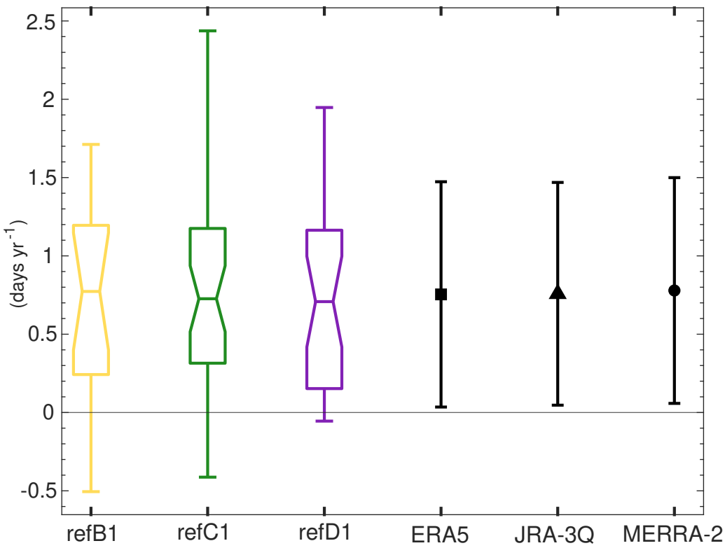
Trends in FWD 50 hPa 1980-1999
