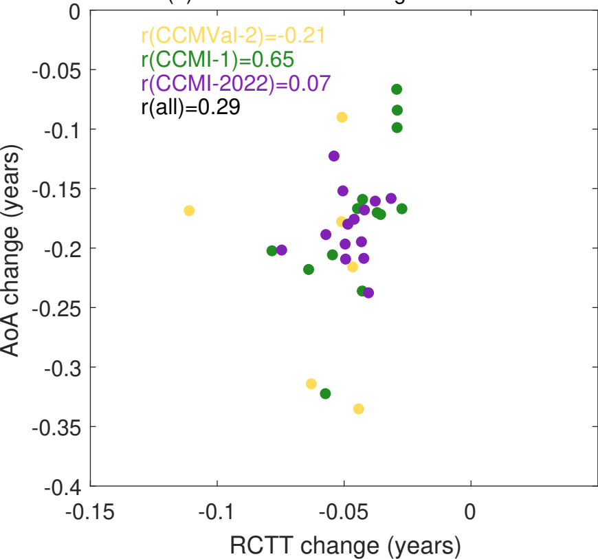
(a) AoA vs. RCTT change 50-20 hPa
