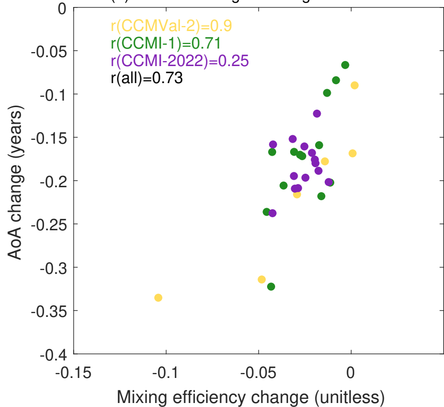
(b) AoA vs. mixing eff change 50-20 hPa
