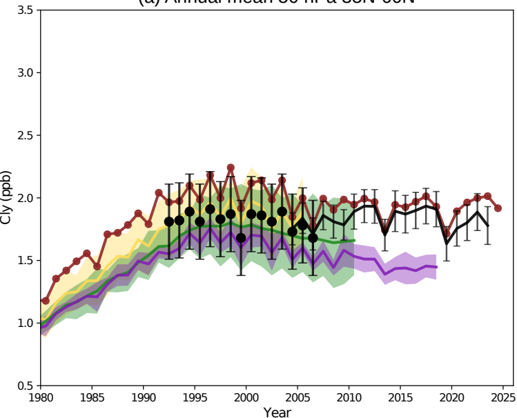
(a) Annual mean 50 hPa 35N-60N
