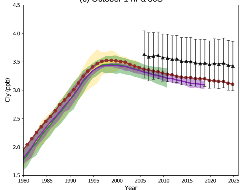
(c) October 1 hPa 80S
