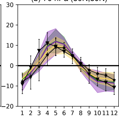
(b) 70 hPa (50N, 89N)
