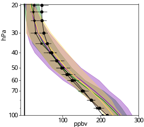
(c) SON (88S, 78S)
