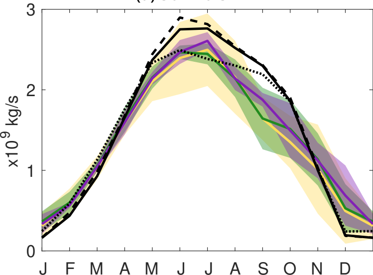
(a) 30 hPa SH
