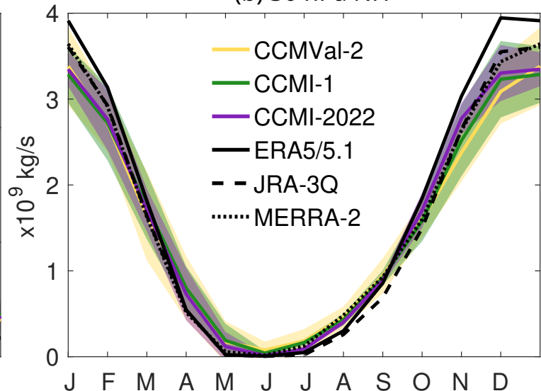
(b) 30 hPa NH
