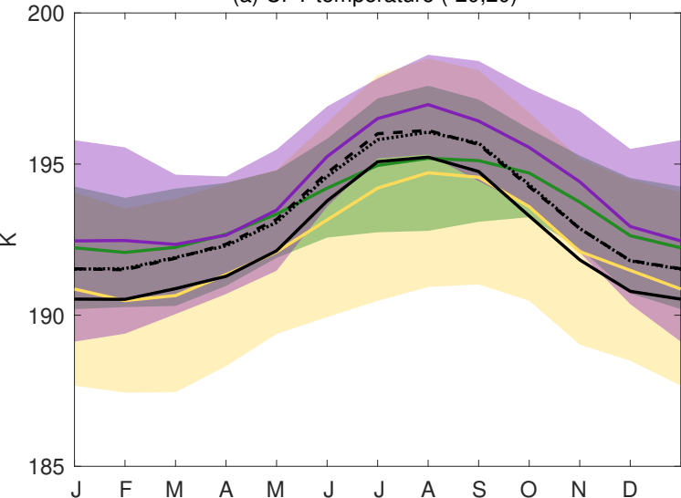
(a) CPT temperature (-20,20)
