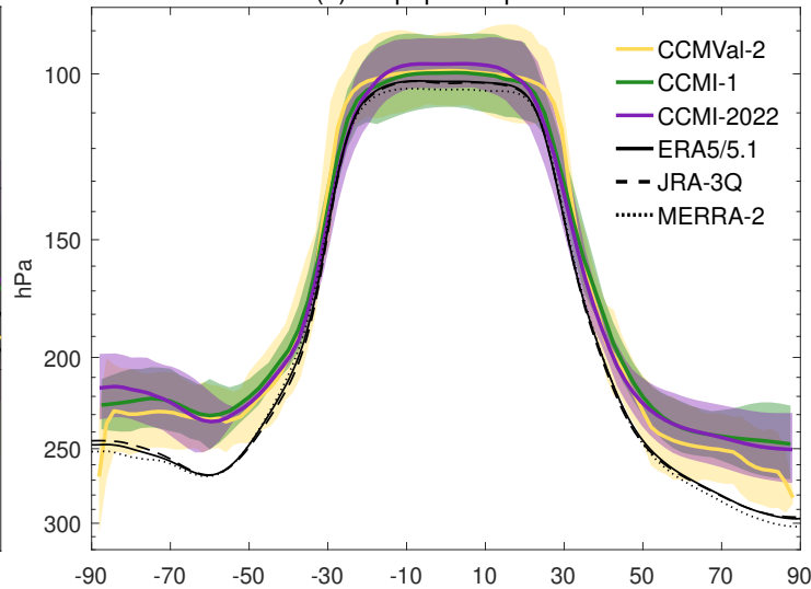
(b) Tropopause pressure
