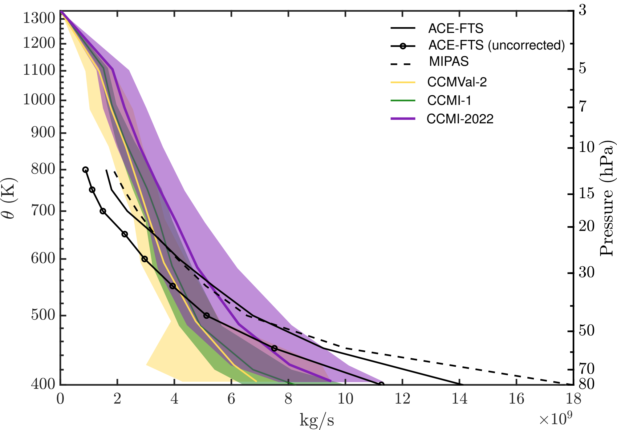
Overturning mass flux from mean age meridional gradient
