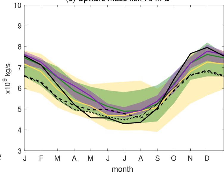
(b) Upward mass flux 70 hPa
