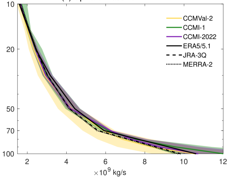
(a) Upward mass flux
