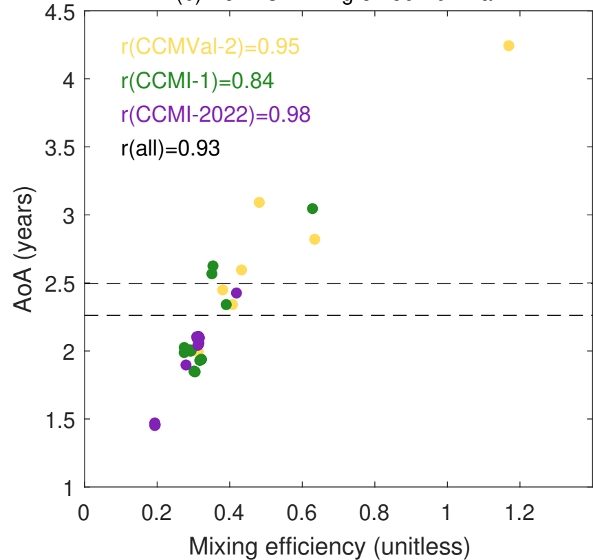
(b) AoA vs. mixing eff 50-20 hPa
