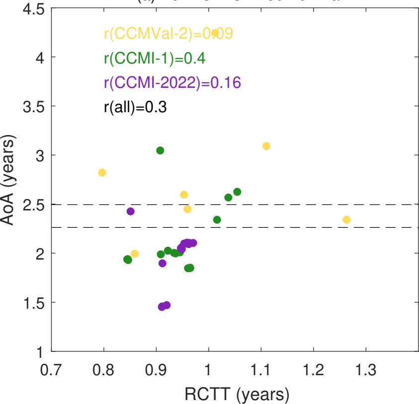
(a) AoA vs. RCTT 50-20 hPa
