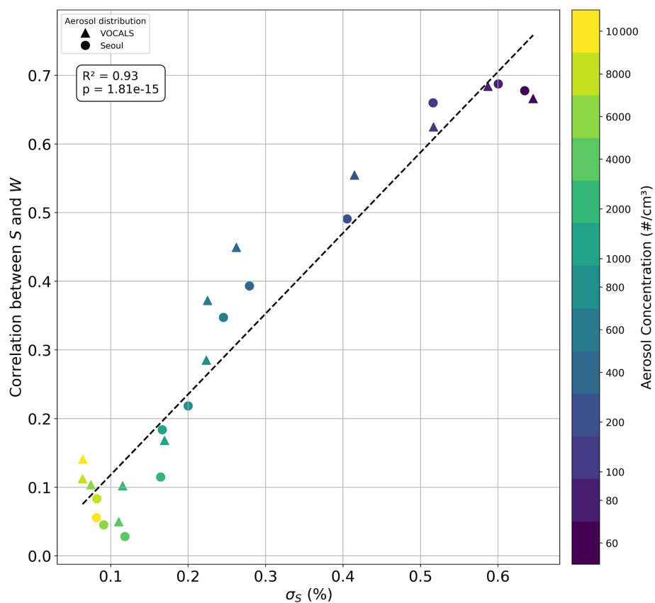
Figure 7. Similar to Fig. 4, except showing the relationship between the domain-averaged supersaturation standard deviation ( \sigma_S ) and the correlation coefficient between supersaturation ( S ) and vertical velocity ( W ), computed at the chamber mid-level ( z = 1.0 m).
