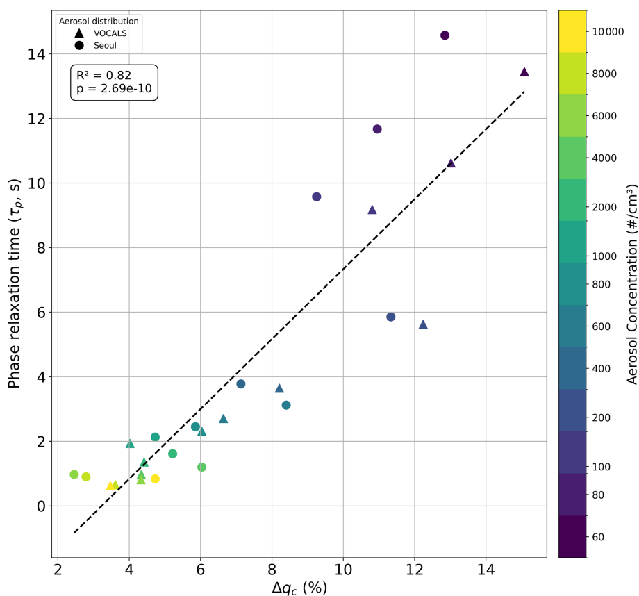
Figure 4. Scatter plot showing the relationship between \Delta q_c (%) and phase relaxation time ( \tau_p ) for VOCALS (triangles) and Seoul (circles) aerosol cases. Each point represents the averaged value for the quasi-equilibrium period (15–30 min).
