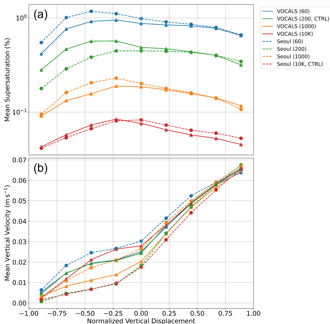
Figure 13. Same as Fig. 12, except for (a) mean S and (b) mean W .
