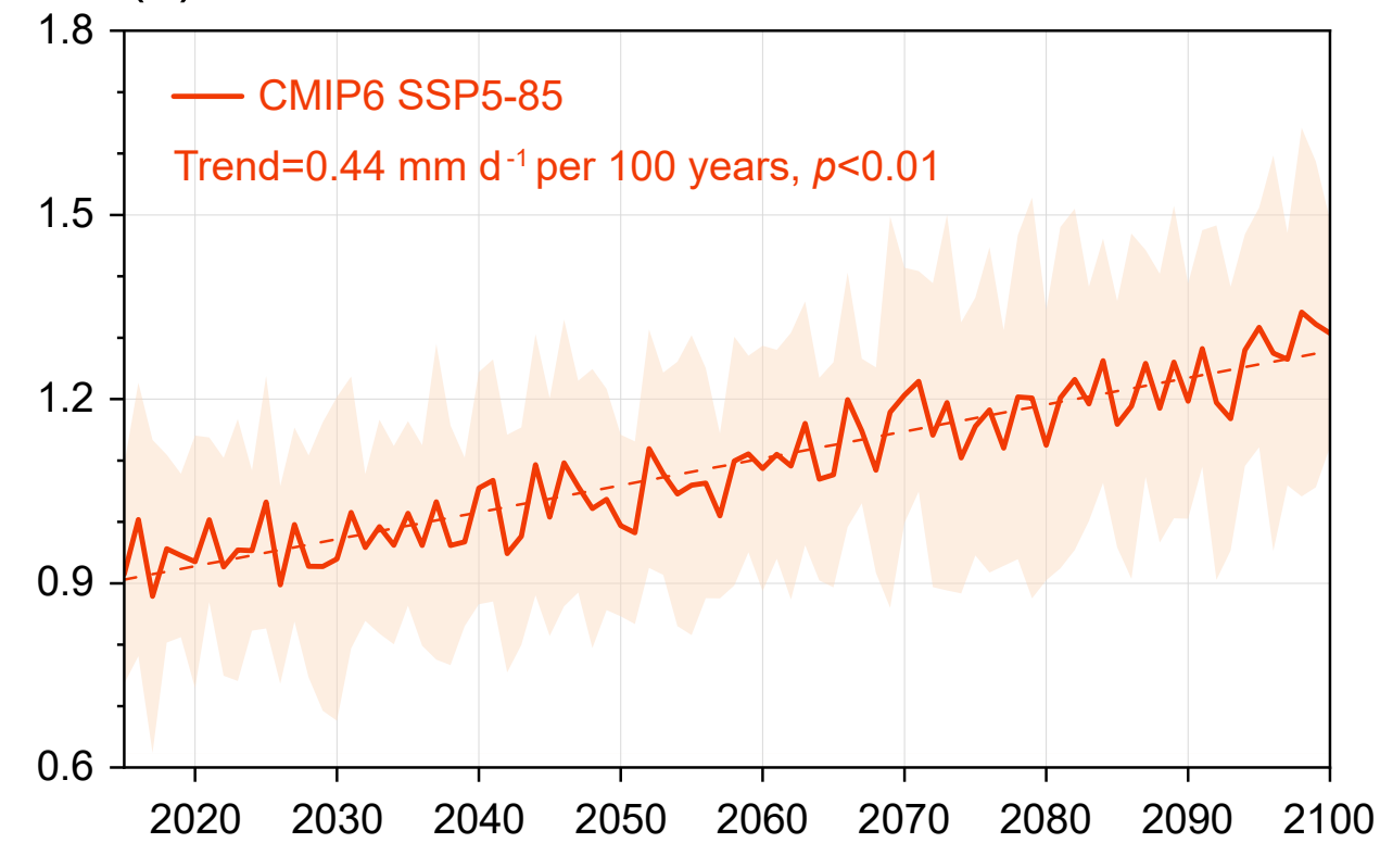
(c) SSP5-85 DJF
