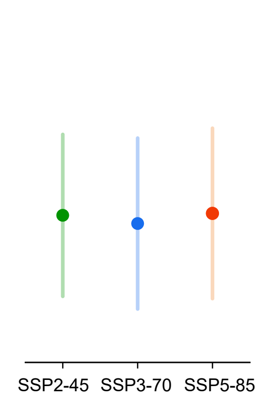
(h) 2091-2100 mean in JJA
