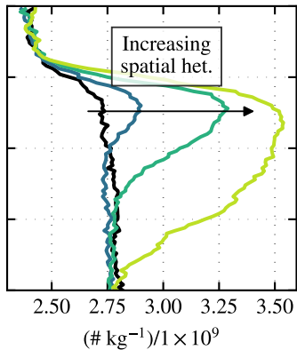
CCN ( S_{\text{env}} = 0.3\% )
