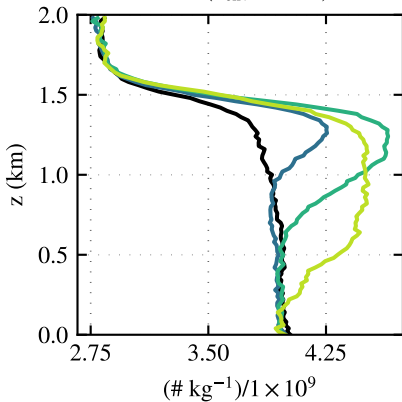
CCN ( S_{\text{env}} = 0.6\% )
