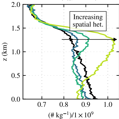
CCN ( S_{\text{env}} = 0.1\% )
