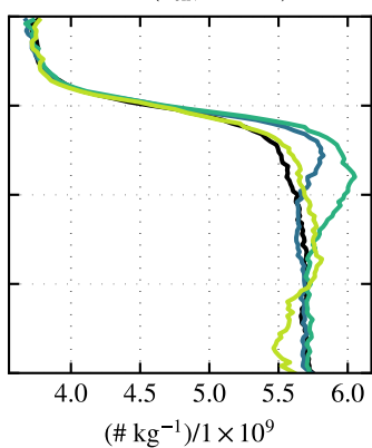
CCN ( S_{\text{env}} = 1.0\% )
