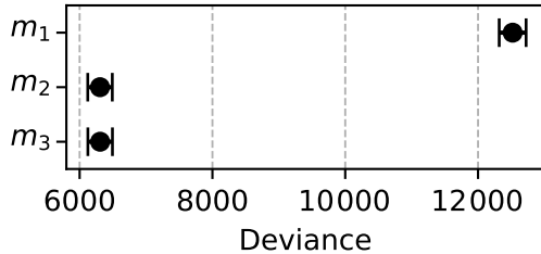
Dataset S_{m_2}
