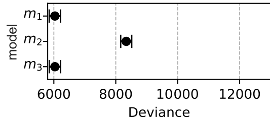
Dataset S_{m_1}
