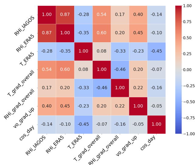
Figure 3. Correlation matrix showing the relationships between selected engineered features, the target variable \text{RH}_i\text{IAGOS} , and the initial ERA5 estimate. The engineered gradient features show a relatively strong correlations with the target \text{RH}_i\text{IAGOS} . The time embeddings ( \text{cos\_day} ) exhibit low direct correlation with \text{RH}_i\text{IAGOS} .
