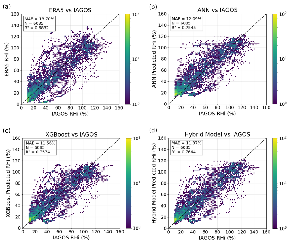
Figure 4. Comparison of RH_i predictions between different models with respect to the target value ( RH_i\_IAGOS ). (a) presents the baseline ERA5 reanalysis, (b) ANN model, (c) XGBoost model, and (d) the hybrid ensemble model. All predictions are made on the test dataset between 400 and 200 hPa over the North Atlantic region (cf. Fig. 1) for the year 2022.
