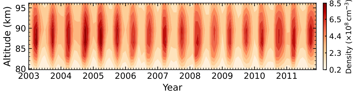
(c) O 3
