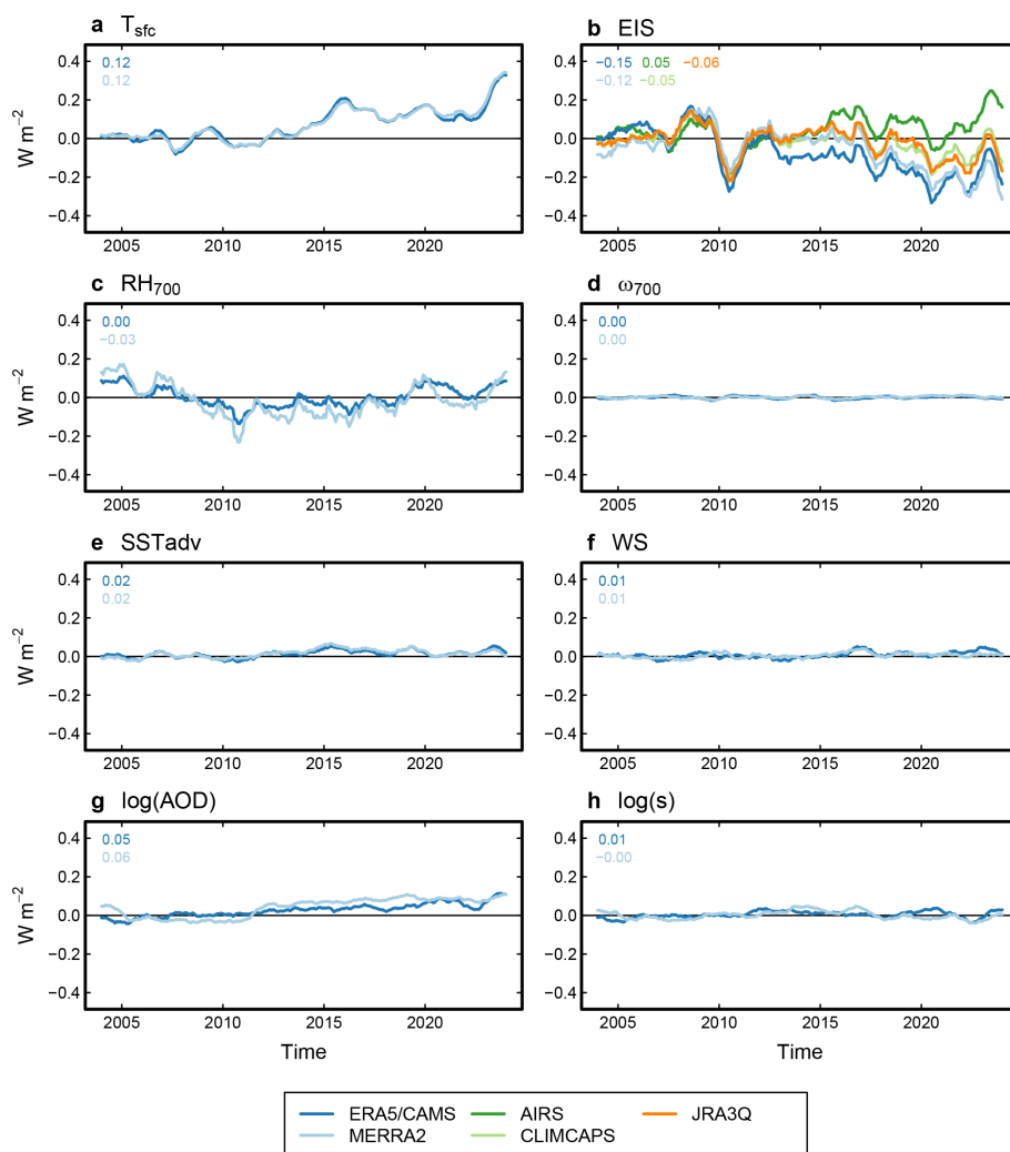
Figure A5. (a–h) As in Fig. A4, but showing the contributions of each CCF dataset to the near-global \text{SWCRE}_{\text{low}} anomalies, calculated relative to the mean of the first 10 years. Decadal trend values (in \text{W m}^{-2} per decade) are shown in the top left corner of each panel. Curves are averages over the corresponding ensemble members: for example, the dark blue curve in (a) is an average over estimates based on every possible combination of five EIS datasets, four aerosol datasets, and ERA5 data for the remaining five CCFs, yielding 20 ensemble members.
