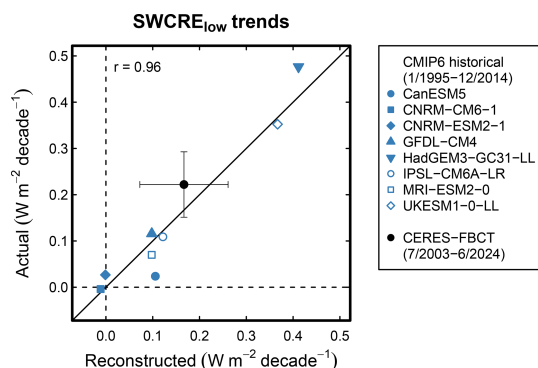
Figure 4. Comparison of actual and reconstructed trends in \text{SWCRE}_{\text{low}} . Blue symbols denote trends from individual CMIP6 models in the historical simulations during January 1995 to December 2014. The black circle shows CERES-FBCT values for July 2003 to June 2024, with error bars denoting \pm 1\sigma confidence intervals. The one-to-one line is shown in solid black.
