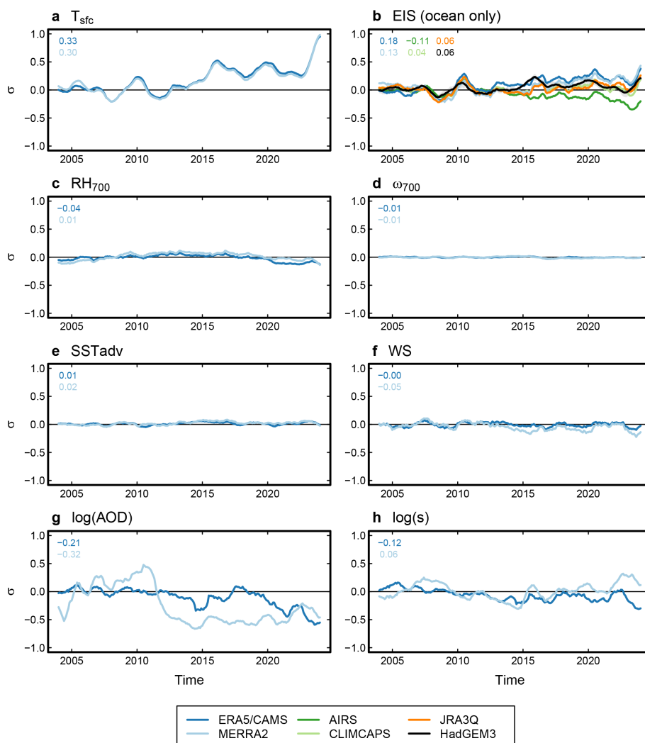
Figure A4. (a–h) Observational estimates of cloud-controlling factor (CCF) anomalies. Timeseries show standardised, deseasonalised monthly anomalies relative to the mean of the first 10 years, smoothed with a 12-month centred running mean; decadal trend values (in \sigma per decade) are shown in the top left corner of each panel. For each variable, the standardisation is done using the ERA5 or CAMS standard deviation, so that the magnitudes are comparable across datasets. Values are near-global averages ( 60^\circ S to 60^\circ N). In (b), in addition to four observational estimates, we include values simulated by a five-member ensemble of extended amip simulations with the HadGEM3 climate model (not used in the CCF analysis). The HadGEM3 ensemble mean is shown in thick black, with grey shading denoting the ensemble range.
