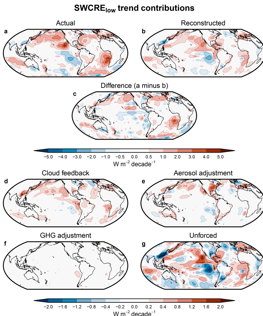
Figure 3. Maps of CERES-FBCT SWCRE low trends, decomposed into contributions. (a) Actual SWCRE low trend, (b) reconstructed trend (sum of panels d–g), (c) difference (a minus b), and contributions from (d) cloud feedback, (e) aerosol adjustment, (f) greenhouse gas (GHG) adjustment, and (g) unforced variability. The GHG adjustment trend contribution (f) is repeated in Fig. A3 with a finer colourbar.
