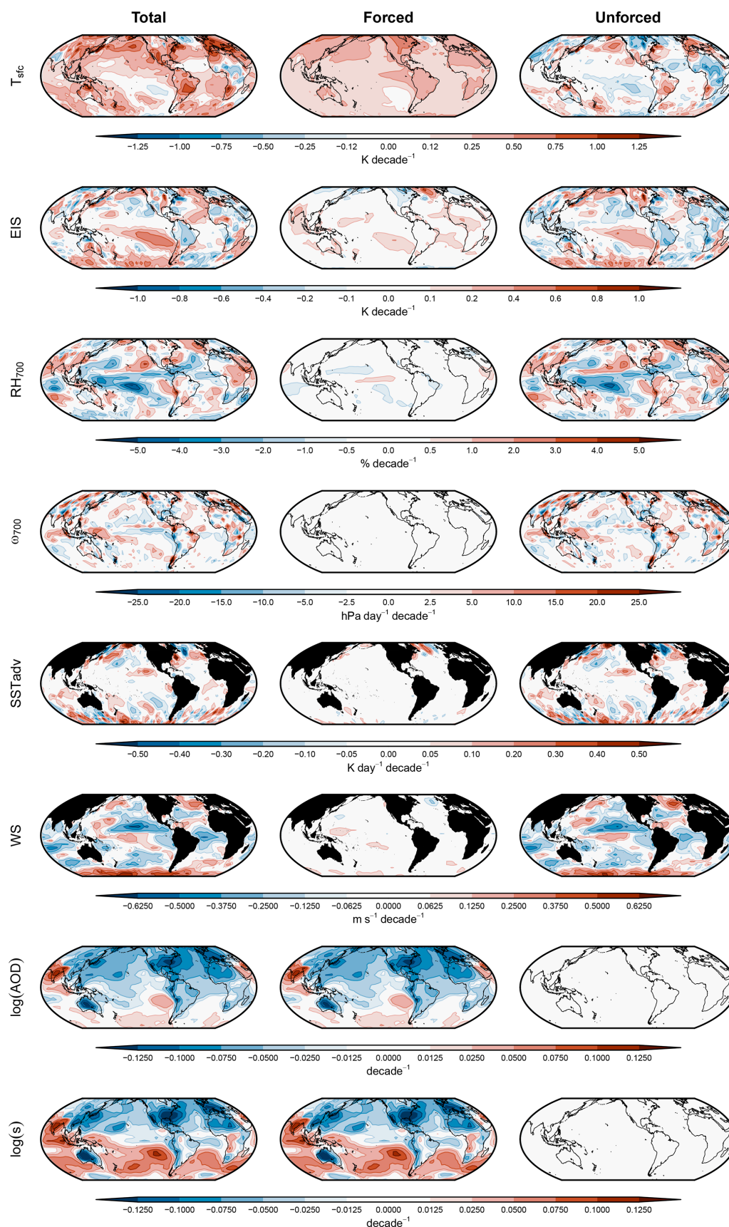
Figure A2. Maps of the decadal trends in each cloud-controlling factor (CCF), representing average values across all CCF datasets (Fig. A4).
