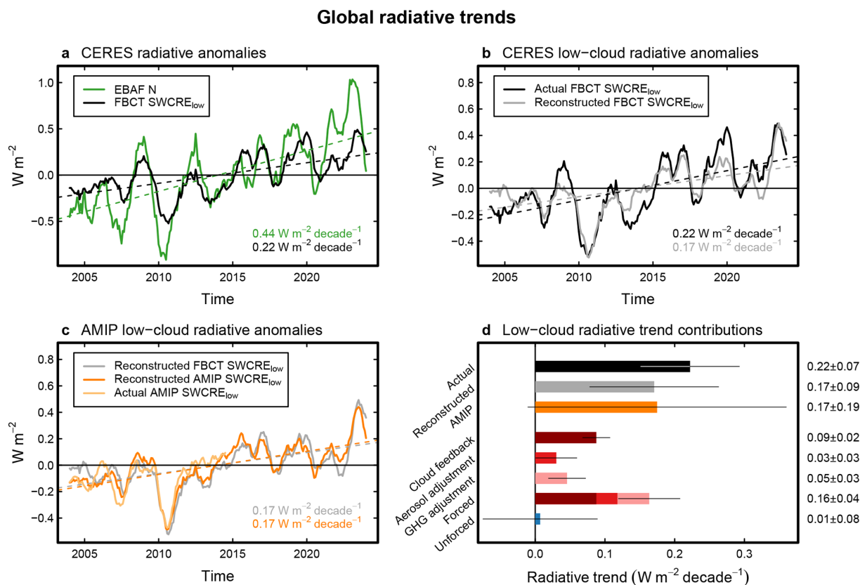
Figure 1. (a–c) Timeseries of global radiative anomalies: (a) CERES-EBAF net radiative imbalance N (green) and CERES-FBCT SWCRE low (black); (b) CERES-FBCT SWCRE low (black) and reconstructed timeseries (grey); (c) reconstructed CERES-FBCT SWCRE low (grey) and CMIP6 SWCRE low (Table A1), emulating extended amip simulations (dark orange). The actual SWCRE low from amip simulations up to December 2014 is shown in light orange. (d) CERES-FBCT actual and reconstructed trends, amip emulated trend, and contributions to the CERES-FBCT reconstructed trend from cloud feedback, aerosol adjustment, greenhouse gas (GHG) adjustment, and unforced climate variability. Thick bars denote central estimates, while thin bars provide \pm 1\sigma ranges. Timeseries show monthly anomalies from the time mean, smoothed with a 12-month centred running mean. Coloured dashed lines represent linear fits to the corresponding timeseries, with trend values (in W m^{-2} per decade, calculated before smoothing the timeseries) shown in the bottom right corner of each panel. Values are near-global averages ( 60^{\circ} S to 60^{\circ} N ), scaled to the global area, except for N which uses global data.
