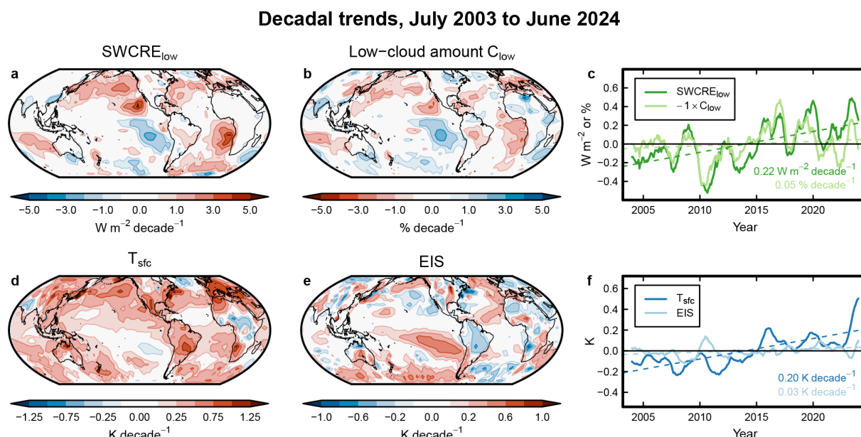
Figure 2. Observed decadal trends in (a) low-cloud radiative effect SWCRE low , (b) low-cloud amount C low (note the inverted colourbar), (d) surface temperature T sfc , and (e) estimated inversion strength EIS (lower-tropospheric stability LTS over land). (c, f) Near-global time-series of the same quantities, averaged from 60° S to 60° N and scaled to the global area. The timeseries show monthly anomalies from the time-mean, smoothed with a 12-month centred running mean. Coloured dashed lines represent linear fits to the corresponding timeseries, with trend values (in W m -2 per decade, % per decade or K per decade, calculated before smoothing the timeseries) shown in the bottom right corner of each panel. Trend maps for other controlling factors are shown in Fig. A2.
