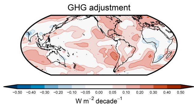
Figure A3. Contribution of GHG adjustments to the \text{SWCRE}_{\text{low}} trend, as in Fig. 3f but with a more finely resolved colourbar.
