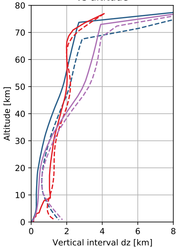
Vertical resolution vs altitude
