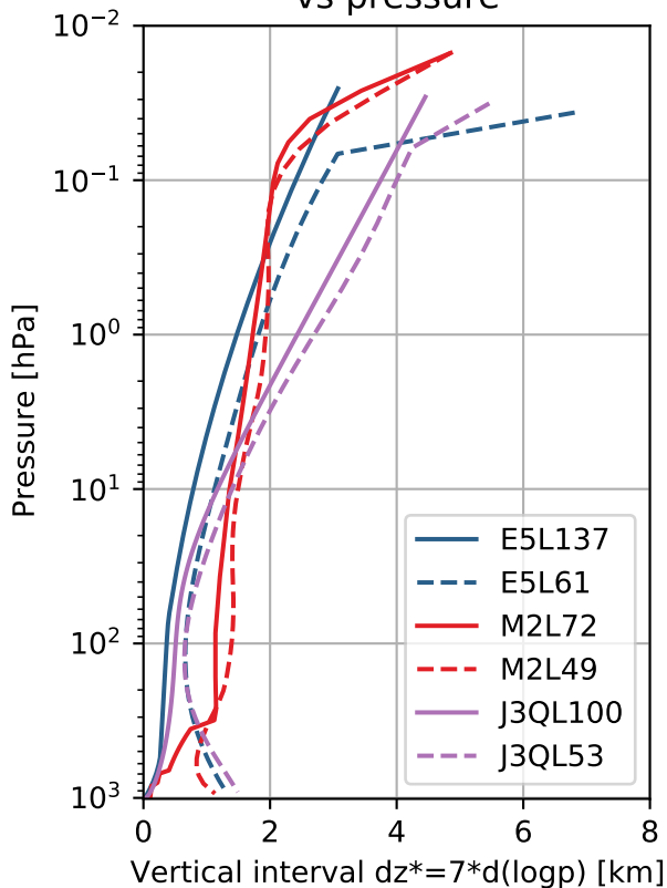
Vertical resolution vs pressure
