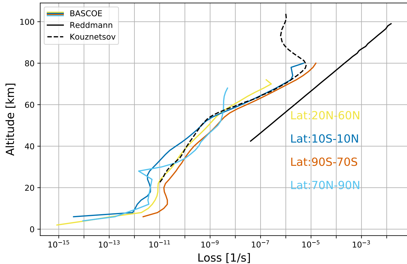
SF 6 loss rate (2002-01-15 12:00)
