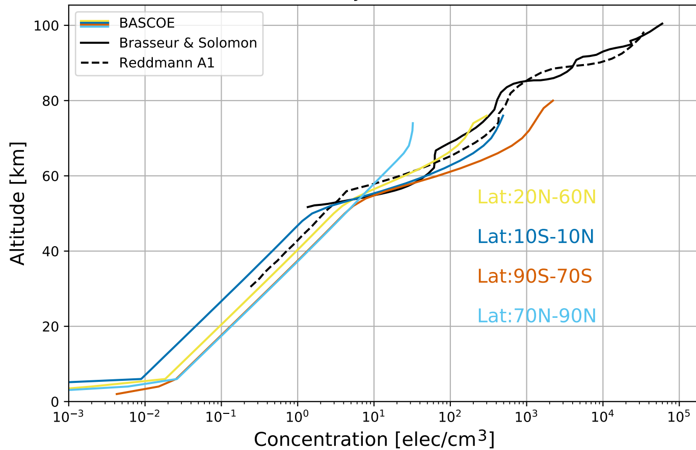
Electron density (2002-01-15 12:00)
