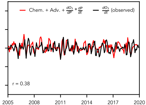
Time-varying tropopause pressure
