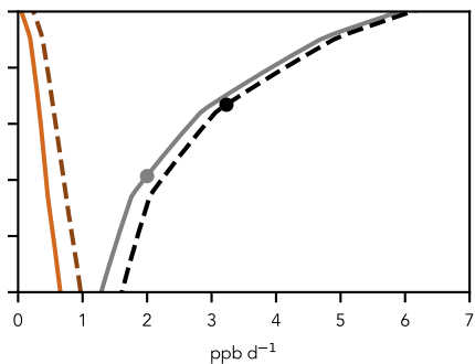
CMAM ozone tendency, RCP 8.5
