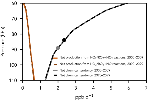
CMAM ozone tendency, RCP 4.5
