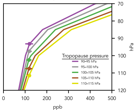
C) Ozone profiles composite by tropopause pressure
