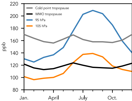
A) Ozone annual cycle (15°S–15°N)
