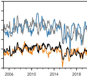
B) Deseasonalized ozone concentrations
