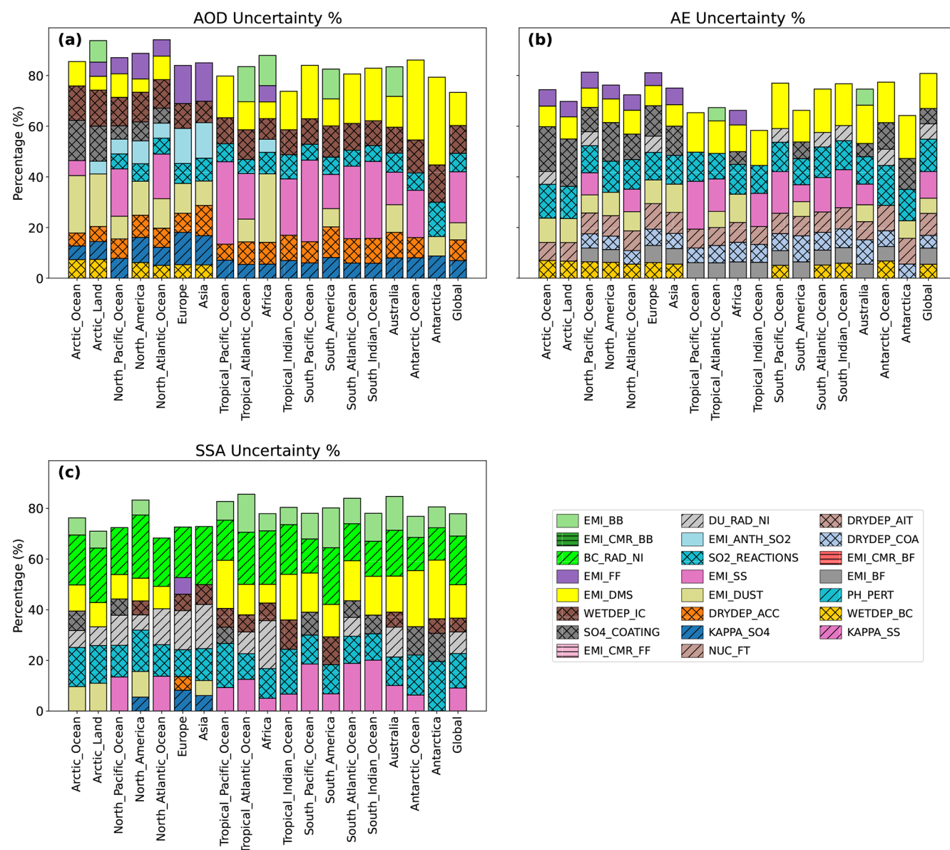
Figure 5. 200 000 model variants and their respective contribution of uncertainties from individual parameters in present-day (a) AOD, (b) AE, (c) SSA. Only parameters above 5 % are shown. No hatches represent parameters perturbing aerosol emissions. Diagonal hatching represents microphysics parameters, crossed hatches represent chemistry perturbing parameters, and horizontal hatches show the emitted diameter-sized parameters.
