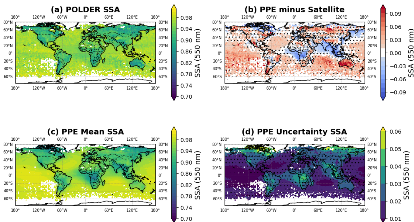
Figure 8. As in Fig. 7 but showing Single Scattering Albedo. Global annual mean Single Scattering Albedo for (a) POLDER instrument measurement, (c) PPE (co-located in space/time at 3-hourly intervals), and (b) the difference between the co-located PPE and POLDER (panel c minus panel a). The spatial magnitude of parametric uncertainty is shown as (d) PPE absolute uncertainty ( 2\sigma across the ensemble members). Stippling indicates where the difference is not statistically significant at the (95 % level of confidence, Student's t -test).
