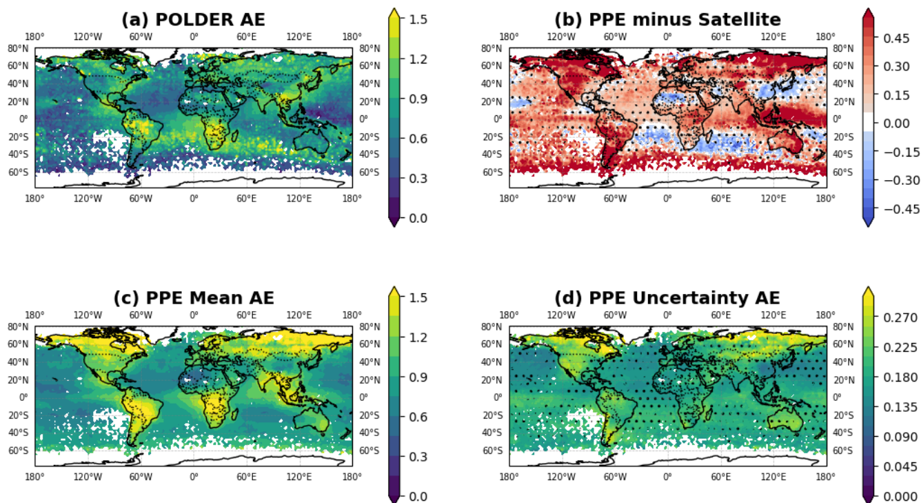
Figure 7. As in Fig. 6, but showing Ångström Exponent. Global annual mean Ångström Exponent for (a) POLDER instrument measurement, (c) PPE (co-located in space/time at 3-hourly intervals), and (b) the difference between the co-located PPE and POLDER (panel c minus panel a). The spatial magnitude of parametric uncertainty is shown as (d) PPE absolute uncertainty ( 2\sigma across the ensemble members). Stippling indicates where the difference is not statistically significant at the (95 % level of confidence, Student's t -test).
