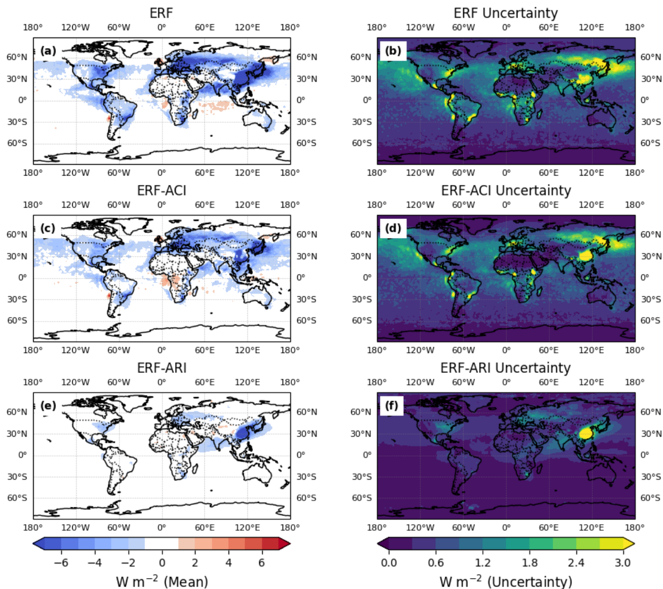
Figure 2. Annual emulated mean (a) ERF, (c) ERF aci , (e) ERF ari and 2 * standard deviation ( 2\sigma ) (b) ERF, (d) ERF aci , (f) ERF ari . 3 million model variants are used to calculate the mean and standard deviation.
