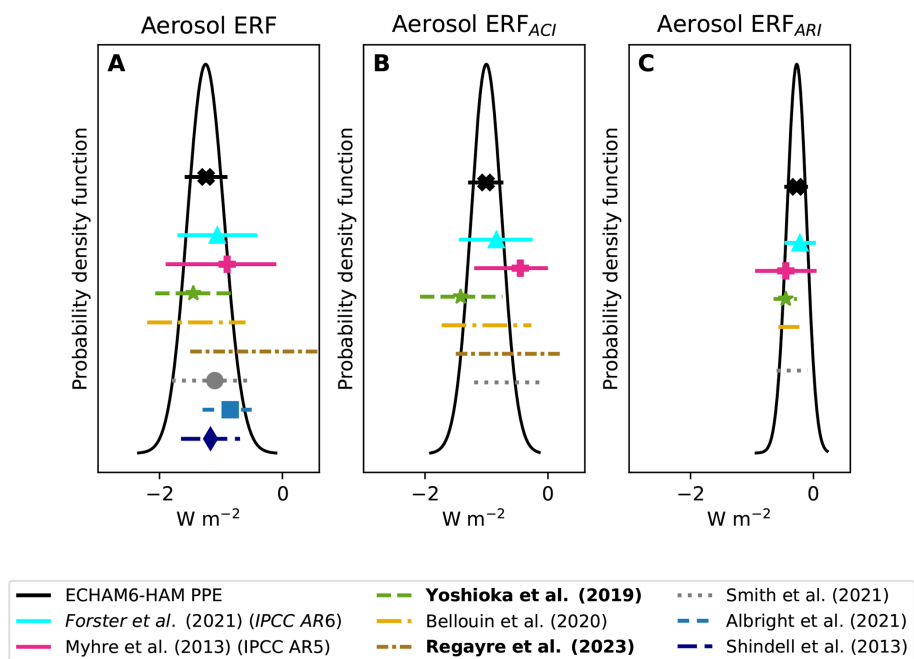
Figure 1. Global annual mean probability density functions between 1850 to 2010 of (a) effective radiative forcing (ERF), (b) \text{ERF}_{\text{aci}} , (c) \text{ERF}_{\text{ari}} from perturbing aerosol parameters. 3 million model emulator-derived variants are used. Our 90 % credible range is shown by the black line with the “X” marker presenting the median. Other estimations shown are using 90 % credible ranges, with their marker representing their respective medians (Myhre et al., 2013; Yoshioka et al., 2019; Bellouin et al., 2020; Regayre et al., 2018; Smith et al., 2021; Albright et al., 2021; Forster et al., 2021). The two perturbed parameter ensemble papers, key motivators here, are highlighted in bold. For Shindell et al. (2013), the 5th to 95th percentile values are calculated as multimodel mean plus and minus standard deviation times 1.645.
