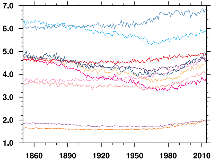
Sulfate Turnover Time (days)
