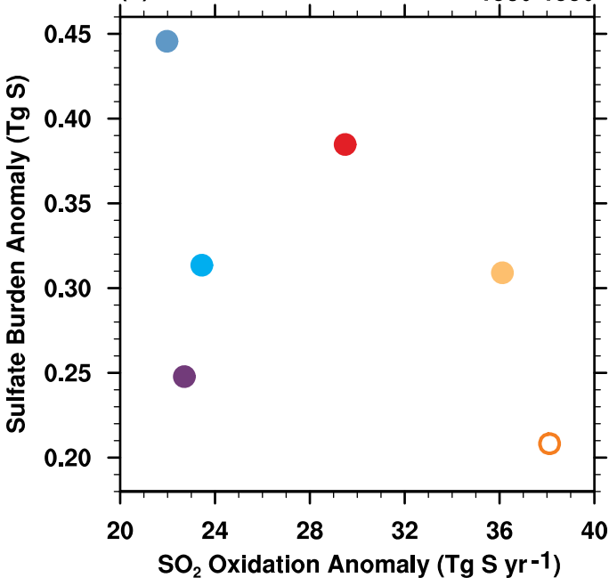
(b) cor = -0.47
