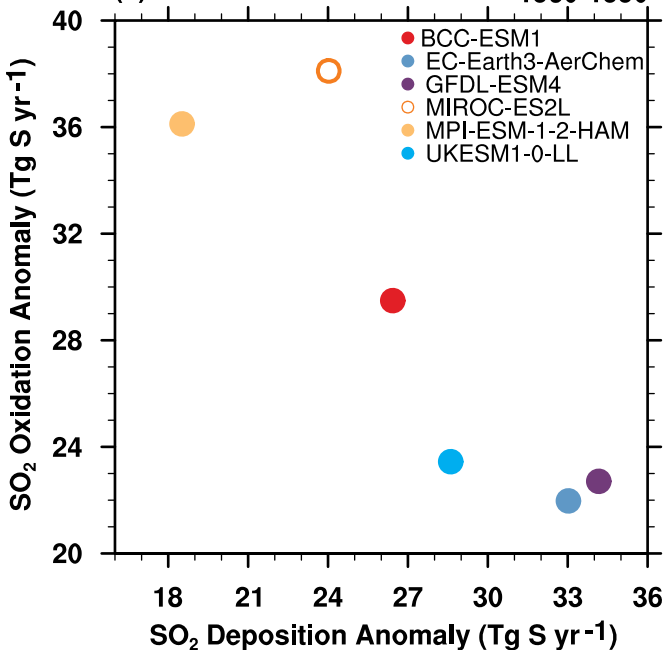
(a) cor = -0.88
