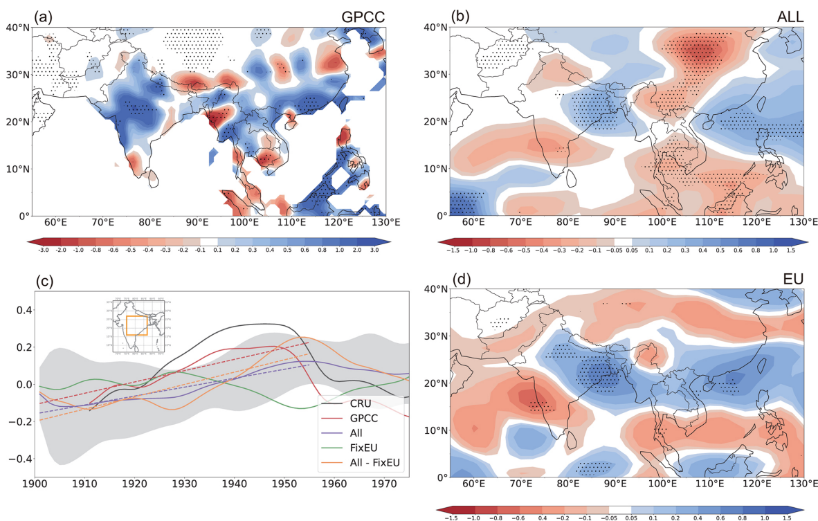
Figure 1. (a–b) Spatial patterns of the 1901–1955 linear trends of JJA precipitation ( \text{mm d}^{-1} (55 \text{ yr})^{-1} ) for (a) GPCC, (b) the all-forcing ensemble (ALL), and (d) the difference between ALL and the all-forcing experiment with fixed preindustrial aerosol emissions over Europe (fixEU), representing the impact of EU aerosols. The black dots mark the grid points for which the trend exceeds the 90 % significance level according to the two-tailed Student's t -test. (c) Time series of area-averaged JJA precipitation anomalies ( \text{mm d}^{-1} ; deviations from the 1901–2000 climatology) over central-northern India (land-only points within 75\text{--}87^\circ \text{ E} , 16\text{--}27^\circ \text{ N} ; area shown in inset map) smoothed with 11-year running means to highlight low-frequency (multi-decadal) fluctuations. The black and red lines represent observations (CRU and GPCC, respectively), while the purple, green and orange lines represent the ensemble means of ALL, fixEU, and their difference (EU). The grey shading represents the standard deviation of the eight-member ALL ensemble around the mean. The 1901–1955 least-squares linear trends of the simulated time series are shown as dashed lines in the corresponding colours. Note that the interval for the simulated changes is half of that used for the observations.
