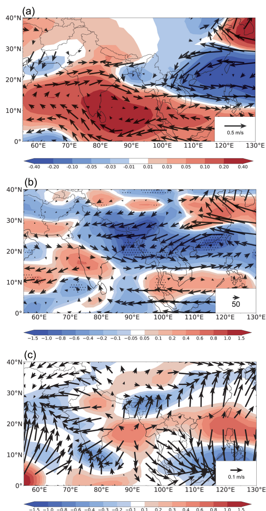
Figure 2. Spatial patterns of the 1901–1955 linear trends of the JJA average (a) 850 hPa winds ( \text{m s}^{-1} (55 \text{ yr})^{-1} ) and 925 hPa streamfunction (colors, 106 \text{ m}^2 \text{ s}^{-1} (55 \text{ yr})^{-1} ), (b) 1000–300 hPa vertically integrated moisture transport (vectors, \text{kg m}^{-1} \text{ s}^{-1} ) and its divergence (shades, \text{mm d}^{-1} (55 \text{ yr})^{-1} ), (c) 150 hPa divergent circulation ( \text{m s}^{-1} (55 \text{ yr})^{-1} ) and its divergence (shades; 10^{-6} \text{ s}^{-1} (55 \text{ yr})^{-1} ) associated with increased European sulphate aerosols (difference between the ALL and fixEU ensemble means). The black dots in (b) mark the grid points for which the trend exceeds the 90 % significance level according to the two-tailed Student's t -test.
