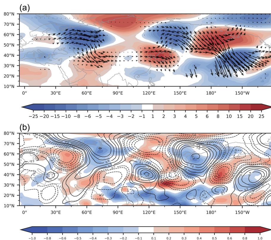
Figure 4. Spatial patterns of the 1901–1955 linear trends of the JJA average (a) 300 hPa wave activity flux (vectors; 10^{-4} \text{ m}^2 \text{ s}^{-2} (55 \text{ yr})^{-1} ) and streamfunction (shades; 10^5 \text{ m}^2 \text{ s}^{-1} (55 \text{ yr})^{-1} ), and (b) 300 hPa meridional wind (contours; \text{m s}^{-1} (55 \text{ yr})^{-1} ) and 500 hPa vertical velocity (shades; 10^{-2} \text{ Pa s}^{-1} (55 \text{ yr})^{-1} ) associated with increased European sulphate aerosols (difference between the ALL and fixEU ensemble means).
