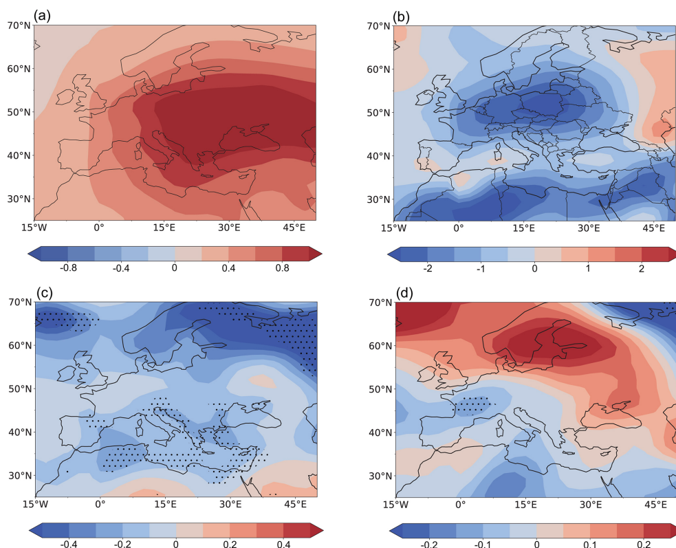
Figure 3. Spatial patterns of the 1901–1955 linear trends of the JJA average (a) column sulphate aerosol burden ( 10^{-5} \text{ kg m}^{-2} (55 \text{ yr})^{-1} ), (b) surface clear-sky downward shortwave radiation ( \text{W m}^{-2} (55 \text{ yr})^{-1} ), (c) 2 m air temperature ( \text{K} (55 \text{ yr})^{-1} ), and (d) sea level pressure ( \text{hPa} (55 \text{ yr})^{-1} ) associated with increased European sulphate aerosols (difference between the ALL and fixEU ensemble means). The black dots in (c) and (d) mark the grid points for which the trend exceeds the 90 % significance level according to the two-tailed Student's t -test.
