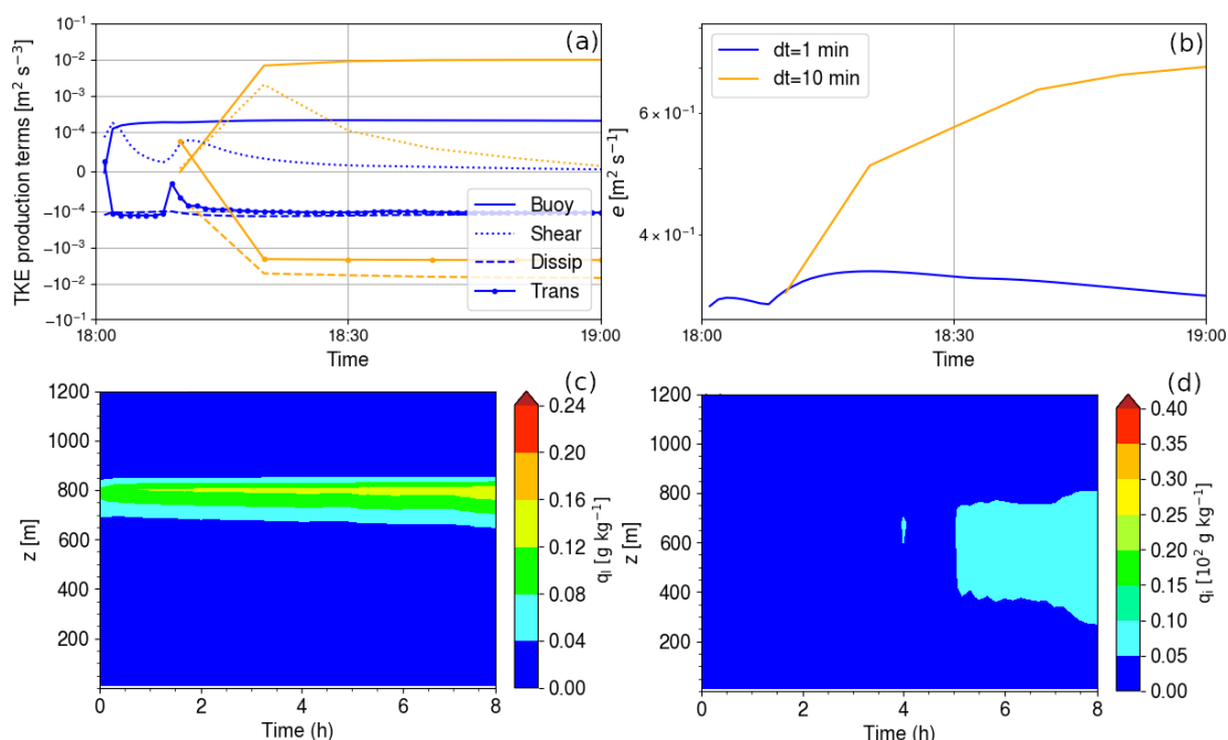
Figure A1. Evolution of the TKE production and loss terms (a) and of the TKE (b) during the first hour of ISDAC simulations at the model level corresponding to cloud top. Yellow (resp. blue) curves correspond to the simulation with a time step of 10 (resp. 1) min. Panels (c) and (d) are the same as Fig. 5c and d but for simulations with a time step of 10 min.
