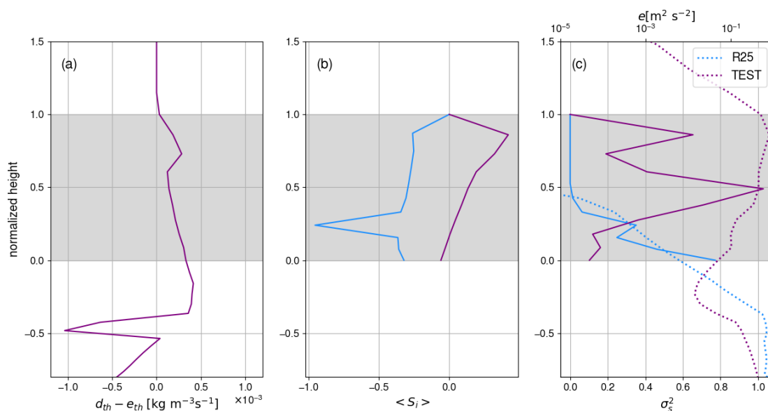
Figure 3. (a) M-PACE Vertical profile of net detrainment rate in the TEST simulation (solid line, bottom x -axis). (b) M-PACE vertical profile of the mean in-cloud supersaturation in the R25 (blue) and TEST (purple) simulation. (c) M-PACE vertical profile of the variance of the in-cloud supersaturation (solid lines, bottom x -axis) and of the TKE in the R25 and TEST simulations (dotted lines, top x -axis). In all panels, the vertical axis is the normalized height and grey shading indicates the cloudy area. The profiles shown correspond to the median profiles over the well-developed phase of the clouds, namely between 01:00 and 05:00 UTC, 10 October 2024.
