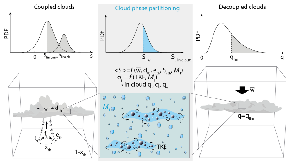
Figure 1. Schematics of LMDZ cloud parameterization and its coupling with the turbulent diffusion and shallow-convection scheme to simulate the phase of polar boundary-layer MPCs. See main text for notations.
