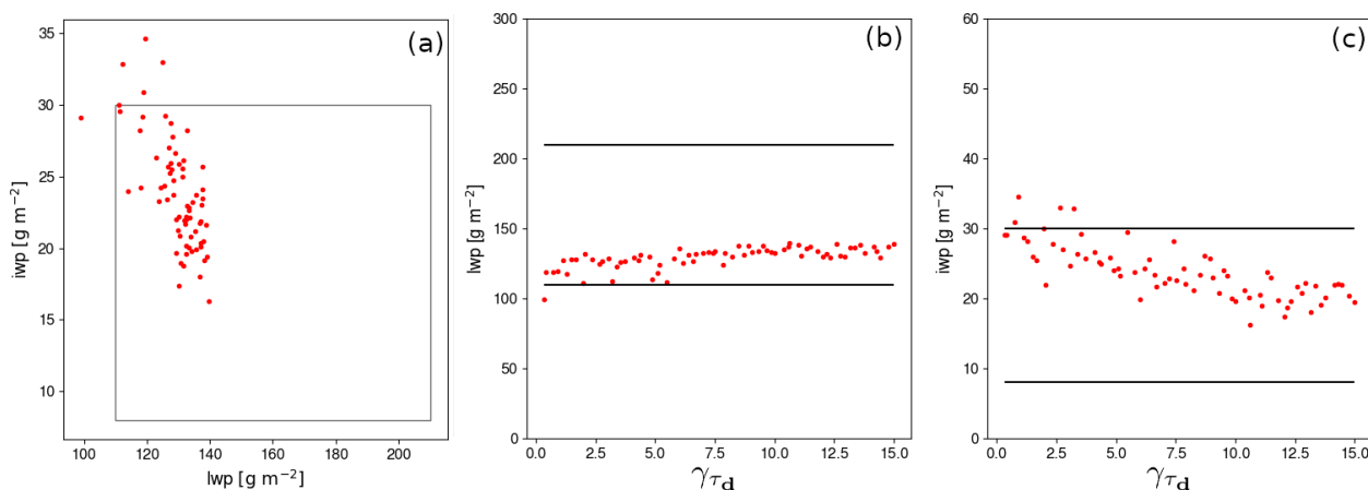
Figure 4. (a) Scatter plot of the mean IWP versus LWP during the well-developed phase of the clouds (between 01:00 and 05:00 UTC, 10 October 2024). Each red dot corresponds to one amongst the 70 members of the M-PACE PPE. In panel (b) (resp. (c)) the LWP (resp. IWP) is plotted versus the value of the \gamma_{\tau_d} parameter (see Eq. 11). The rectangle in panel (a) and the black horizontal lines in panels (b) and (c) indicate the likely range of the regionally averaged LWP and IWP from airborne and ground-based observations according to Klein et al. (2009). Note that the simulated IWP includes the mass of snow precipitation and it considers only the first 2000 m above ground level to avoid accounting for mid- and high-troposphere clouds which can be artefacts as they are not the focus of the case.
