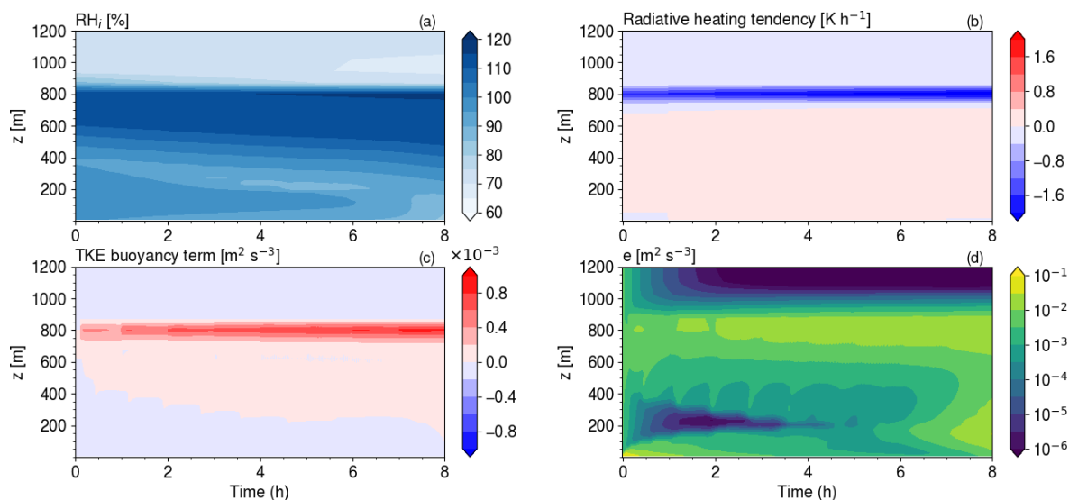
Figure 6. Time height plots of the relative humidity with respect to ice ( a ), radiative heating tendency ( b ), TKE production term by buoyancy ( c ) and TKE ( d ) in the TEST LMDZ SCM simulation on the ISDAC case.
