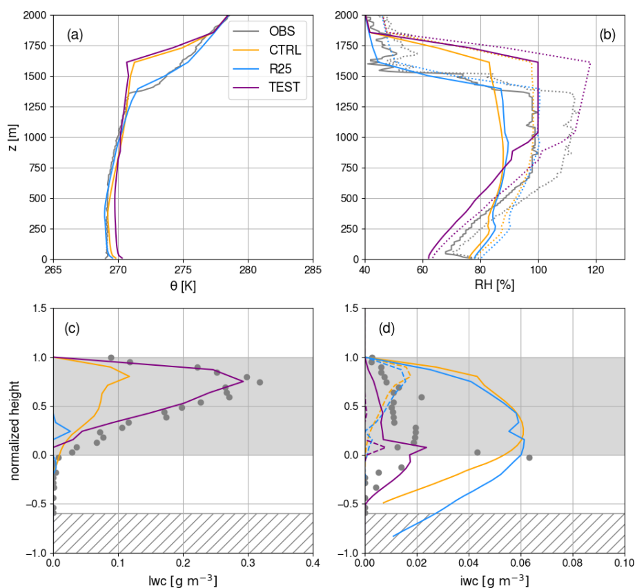
Figure 2. M-PACE vertical profiles of potential temperature (a), relative humidity with respect to liquid ((b), solid lines) and ice ((b), dotted lines), liquid water content (c) and ice water content including (resp. excluding) snow precipitation in solid (resp. dashed) lines (d). CTRL, R25 and TEST simulations are shown in orange, blue and purple respectively and simulation profiles are averaged over the well-developed phase of the clouds, namely between 01:00 and 05:00 UTC, 10 October 2024. In panels (a) and (b), observations (in grey) correspond to the radiosonde launched at Utqiagvik, Alaska at 17:00 UTC, 9 October. In panels (c) and (d), the vertical axis used is the normalized height – where –1 is the surface, 0 is cloud base, and 1 is cloud top – for consistency with Klein et al. (2009) and grey shading indicates the location of the cloud. Observations (grey dots) correspond to airborne measurements that do not extend below –0.6 in normalized height, hence the hashed area in panel (c) and (d). Note that in LMDZ, the relative humidity corresponds to a diagnostic variable computed as the ratio of the mean specific humidity in the mesh to the saturation specific humidity at the mean temperature in the mesh, the relative humidity with respect to liquid being capped at 100 % as cloud liquid water forms through adjustment process.
