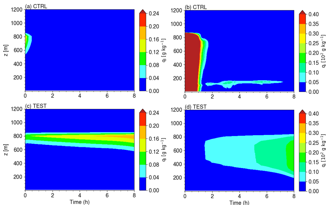
Figure 5. Time-height plot of the specific content of cloud liquid water ( a , c ) and ice water including snow precipitation ( b , d ) in the CTRL ( a , b ) and TEST ( c , d ) LMDZ SCM simulations on the ISDAC case. Colormap and colorbar's levels are the same as those of Fig. 2 in Ovchinnikov et al. (2014) for easy visual comparison with LES results. It is worth recalling that unlike in Ovchinnikov et al. (2014), ice-related processes are allowed from the beginning of the simulations (no 2 h spin-up).
