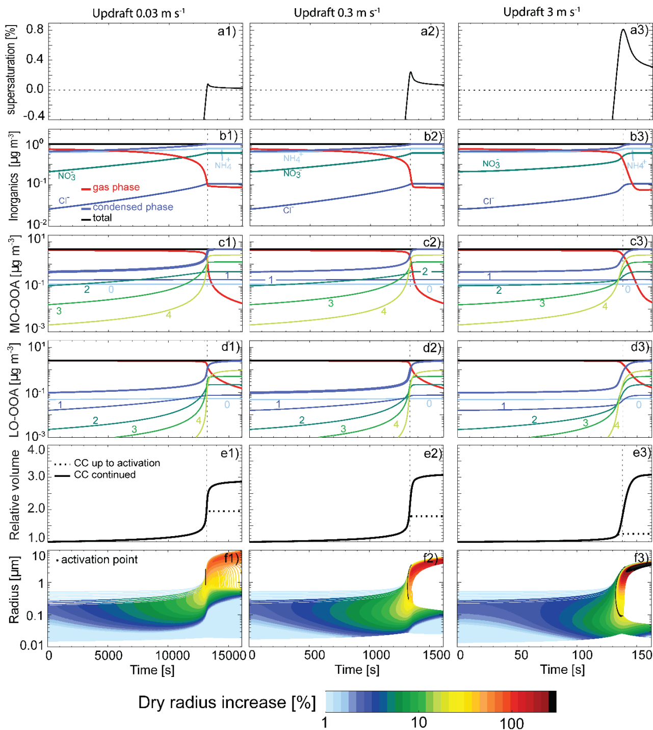
Figure S4. Time series of a) supersaturation, b-d) inorganic and organic species, e) droplet dry volume relative to the initial state 80% RH, f) wet radius, at updraft of 0.03 (left), 0.3 (middle), and 3 m s -1 (right panel) for VBS 2.
