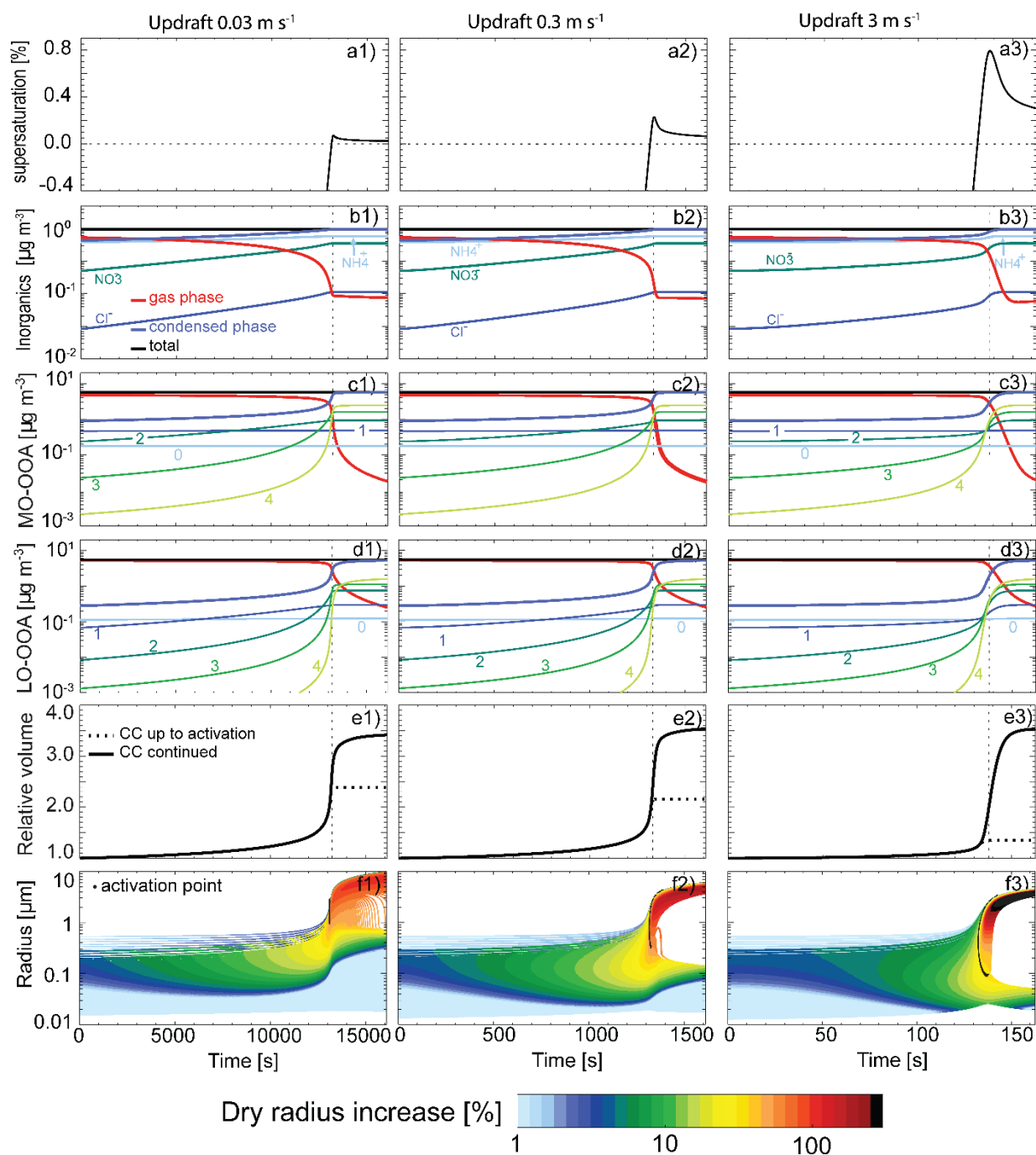
Figure S3. Time series of a) supersaturation, b-d) inorganic and organic species, e) droplet dry volume relative to the initial state of 80% RH, f) wet radius, at updraft of 0.03 (left), 0.3 (middle), and 3 m s -1 (right panel) for VBS 1.
