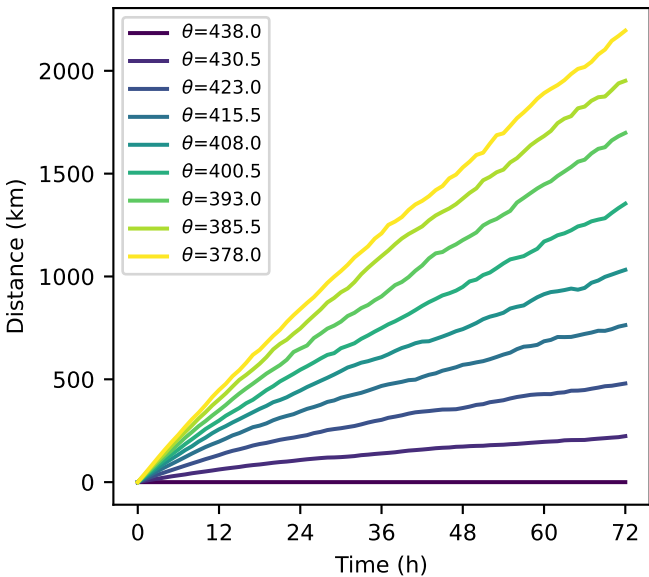
Median distance with \theta=438 K level
