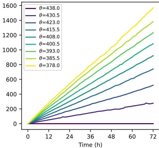
St. dev. of distance with \theta=438 K level
