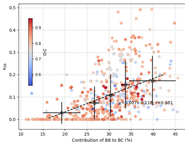
Figure 5. Variation of \kappa_{\text{OA}} as a function of relative contribution of biomass burning to BC ( f_{\text{bb}} ), with colors indicating the corresponding O : C ratios. Black open squares represent binned mean \kappa_{\text{OA}} values based on f_{\text{bb}} bins defined by 20-percentile intervals, with error bars indicating one standard deviation. The dashed line shows a linear regression fitted to the binned means.
