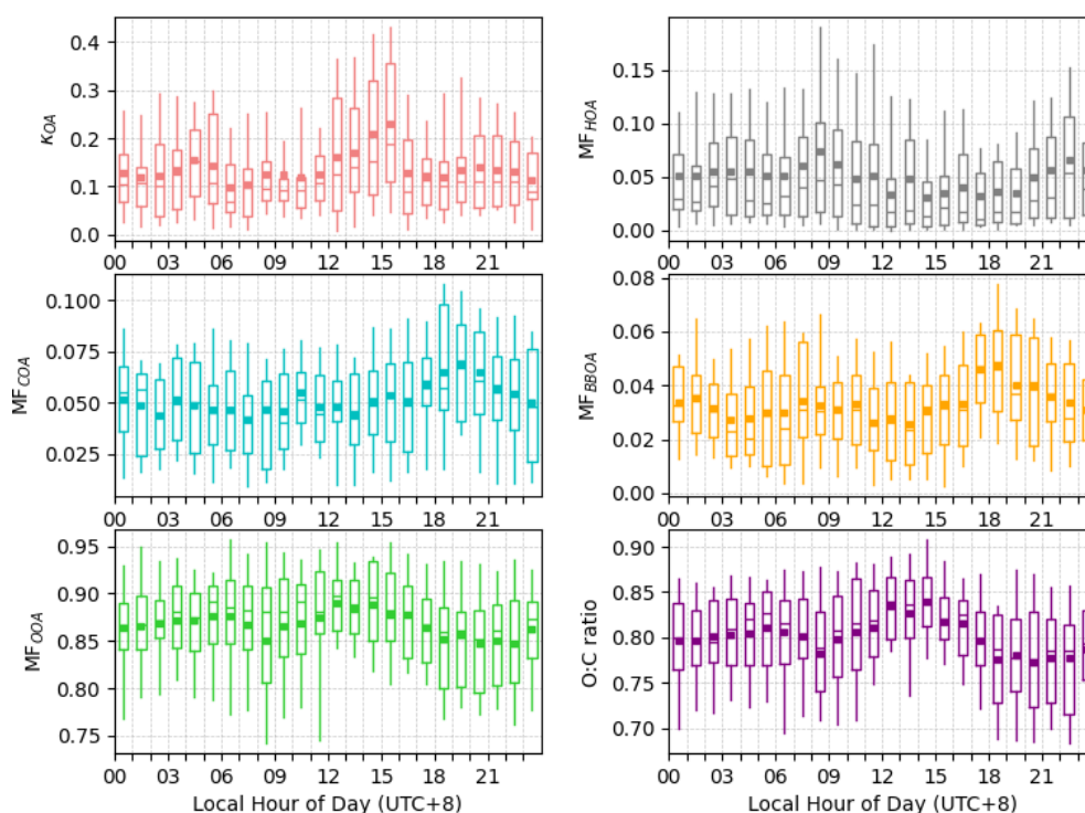
Figure 4. Diurnal variations of \kappa_{\text{OA}} , mass fraction of four OA factors, and O : C ratio during the winter campaign. The upper and lower bounds of each box represent the 75th and 25th percentiles, and the upper and lower whiskers represent the 95th and 5th percentiles. The line in each box is the median value and the square represents the mean.
