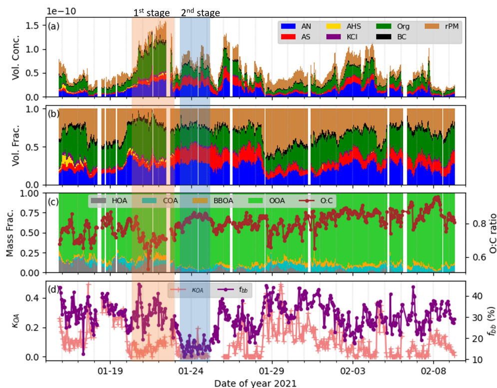
Figure 3. Time series of (a) volume concentrations, (b) volume fractions of different chemical species in \text{PM}_{2.5} , (c) mass fractions of different OA factors and O : C ratio, (d) \kappa_{\text{OA}} and relative contribution of biomass burning to BC ( f_{\text{bb}} ) at the Huainan site during the winter campaign. The shaded area denotes a persistent pollution episode from 20 to 25 January 2021, with different colors indicating distinct stages of the episode.
