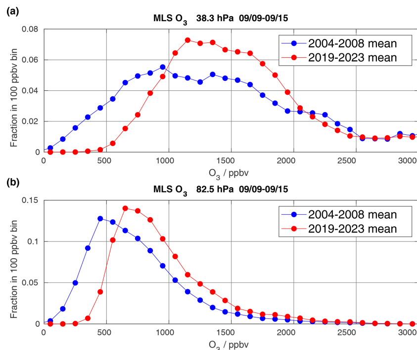
Figure 5. Fraction of the Antarctic vortex-average MLS ozone distributions in each 100 ppbv bin, for the week centered on 12 September for the periods 2004–2008 (blue) and 2019–2023 (red), at (a) 38.3 hPa and (b) 82.5 hPa.
