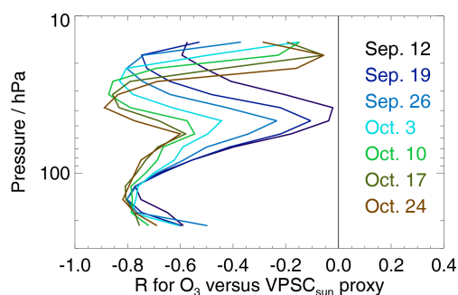
Figure 10. An expanded view of the correlation coefficient ( R ) between the ozone vortex-average time series and the lower stratospheric \text{VPSC}_{\text{sun}} proxy described in the text and in Fig. 8. Results are shown as a function of pressure for each of the September and October weeks considered here, as labeled on the right side of this plot.
