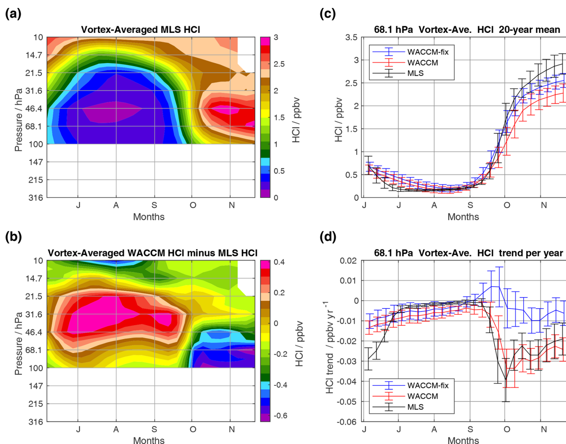
Figure 6. Same as Fig. 3, but for HCl.
