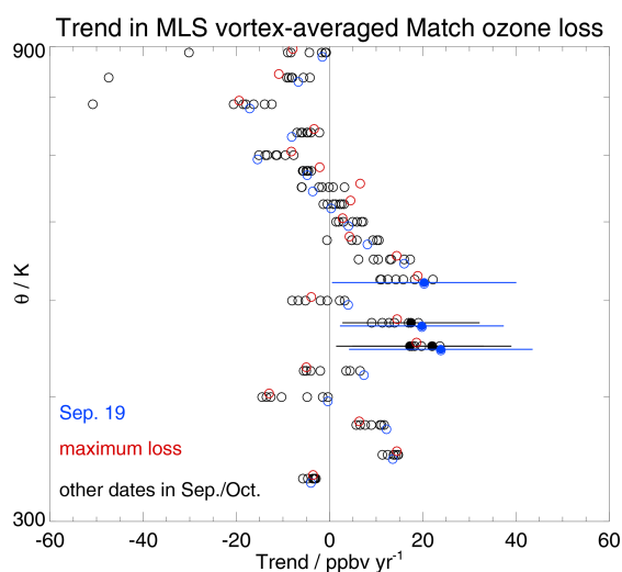
Figure 19. Chemical ozone loss trend profiles inside the Antarctic lower stratospheric vortex from Match-based analyses of MLS data from May through October, for 2005–2023. Only a few trends, marked by the filled circles with associated ( 2\sigma ) error bars, are significant; for clarity, other error bars are omitted. The blue circles are for the week centered on 19 September, the red circles are trends based on the maximum cumulative losses for each year, and the other points (in black) represent trend values for the other analyzed weeks, from 12 September to 24 October.
