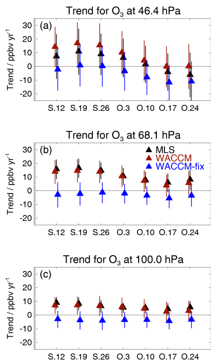
Figure 13. A comparison of the vortex-average trends for 2005–2023 based on MLR analyses from MLS, WACCM, and WACCM-fix-EESC (labeled WACCM-fix) for the weeks from 12 September through 24 October for (a) 46 hPa, (b) 68 hPa, and (c) 100 hPa.
