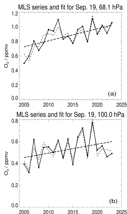
Figure 11. Examples of MLR fits to the MLS vortex-average ozone time series at (a) 68 hPa and (b) 100 hPa for the week centered on 19 September. The MLS ozone averages are given by the solid line, the ozone trend (slope component of the MLR fit) is shown by the thick dashed line, and the thin dashed line gives the full fit from the MLR analysis.
