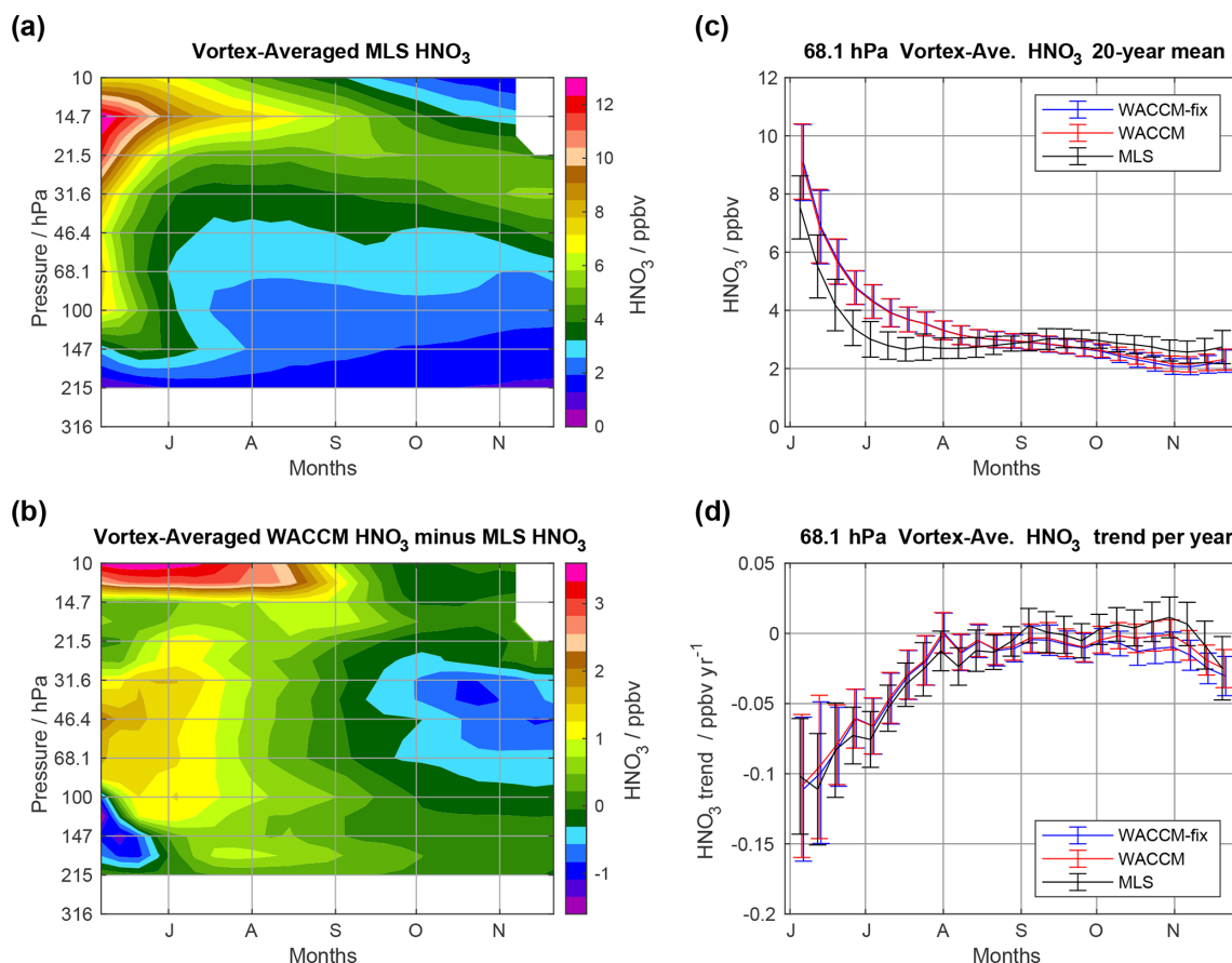
Figure 7. Same as Fig. 3, but for HNO 3 .
