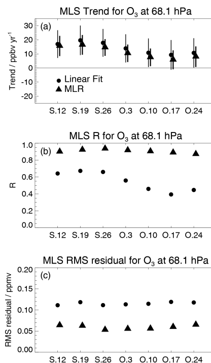
Figure 12. Results at 68 hPa for (a) the trends in MLS vortex-average ozone over Antarctica, (b) the correlation coefficients between the fits and the MLS \text{O}_3 series and (c) the RMS residuals for these fits, as a function of weeks in September and October (centered on 12 September, labeled S.12, to 24 October, labeled O.24). The filled circles and filled triangles represent results from a simple linear fit and MLR, respectively, for 2005–2023. Trend error bars in panel (a) represent 2\sigma .
