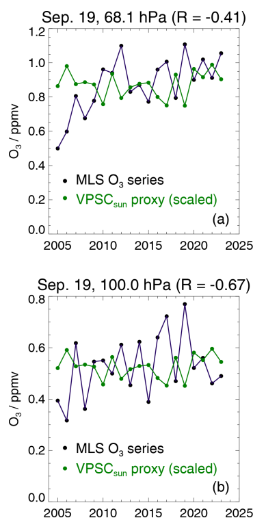
Figure 9. Vortex-average Antarctic ozone variations from MLS (black) over 2005–2023 for the week centered on 19 September at (a) 68 hPa and (b) 100 hPa. The green lines are a scaled version of the variability in the \text{VPSC}_{\text{sun}} proxy term described in the text (in relation to Fig. 8); the scaling (using the average ozone value over the years divided by the average relative change in the proxy) is applied here to show the relative changes in this proxy from year to year on the same scale as the ozone ranges in each panel.
