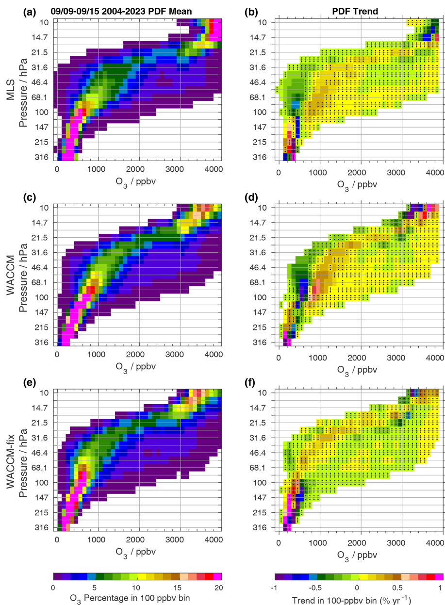
Figure 4. (a) A histogram of all MLS lower-stratospheric vortex O 3 observations from the week of 9–15 September for 2004–2023, normalized separately for each level, representing the underlying PDF. (b) PDF (histogram) trends shown are the slopes from linear fits within each bin to values from histograms prepared as in panel (a), but separately for each year. Bins without black stippling have trends that are larger in magnitude than the 1 uncertainty in the trend. Panels (c) and (d) are the same as panels (a) and (b), respectively, but for the WACCM simulation. Panels (e) and (f) are the same as panels (a) and (b), respectively, but for the WACCM-fix-EESC simulation.
