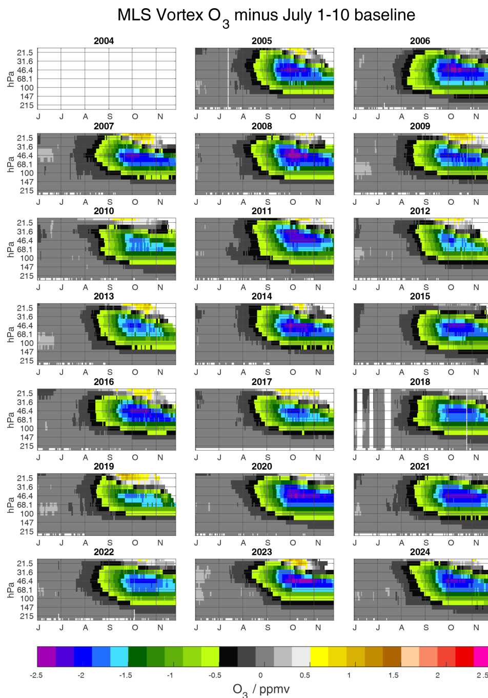
Figure 1. June to November vortex-average lower stratospheric ozone profiles over the range 215–21 hPa for 2005–2024. The respective 1–10 July average is subtracted for each year to remove interannual variability of early-winter (baseline) conditions. Partial 2004 is not included because MLS operations had not begun in July, so this baseline could not be calculated.
