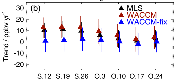
Trend for \Delta O_3 at 68.1 hPa
