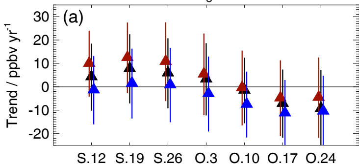
Trend for \Delta O_3 at 46.4 hPa
