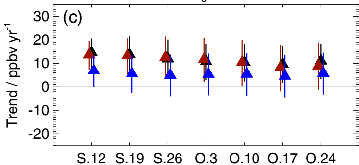
Trend for \Delta O_3 at 100.0 hPa
