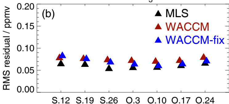
RMS residual for O 3 at 68.1 hPa
