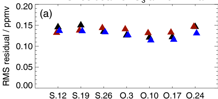
RMS residual for O 3 at 46.4 hPa
