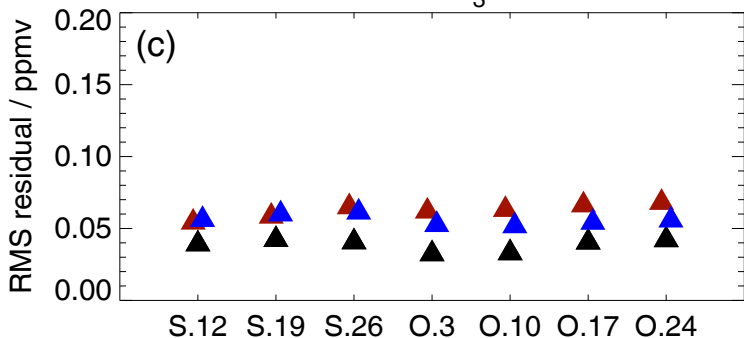
RMS residual for O 3 at 100.0 hPa
