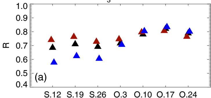
R for O 3 at 46.4 hPa
