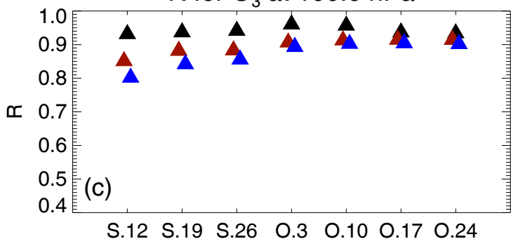
R for O 3 at 100.0 hPa
