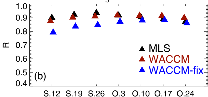
R for O 3 at 68.1 hPa
