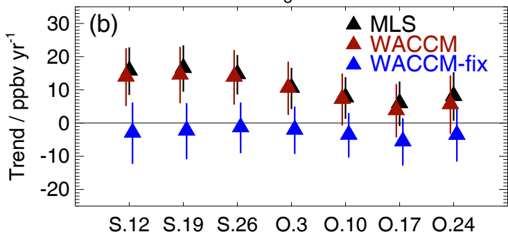
Trend for O 3 at 68.1 hPa
