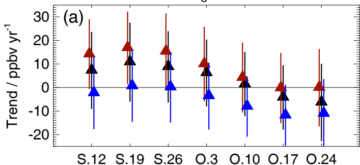
Trend for O 3 at 46.4 hPa
