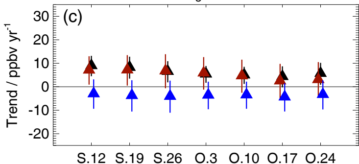
Trend for O 3 at 100.0 hPa
