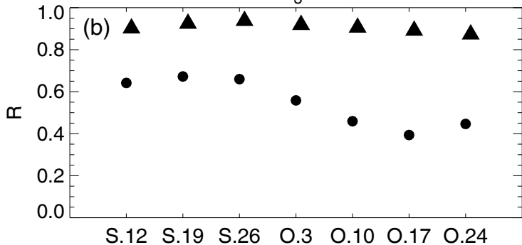
MLS R for O 3 at 68.1 hPa
