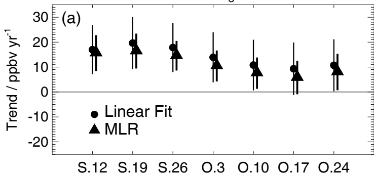
MLS Trend for O 3 at 68.1 hPa
