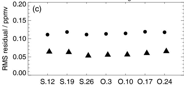
MLS RMS residual for O 3 at 68.1 hPa
