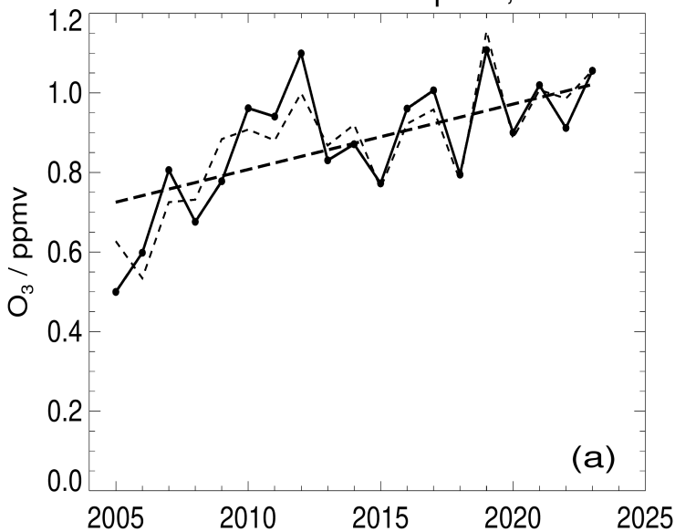
MLS series and fit for Sep. 19, 100.0 hPa
