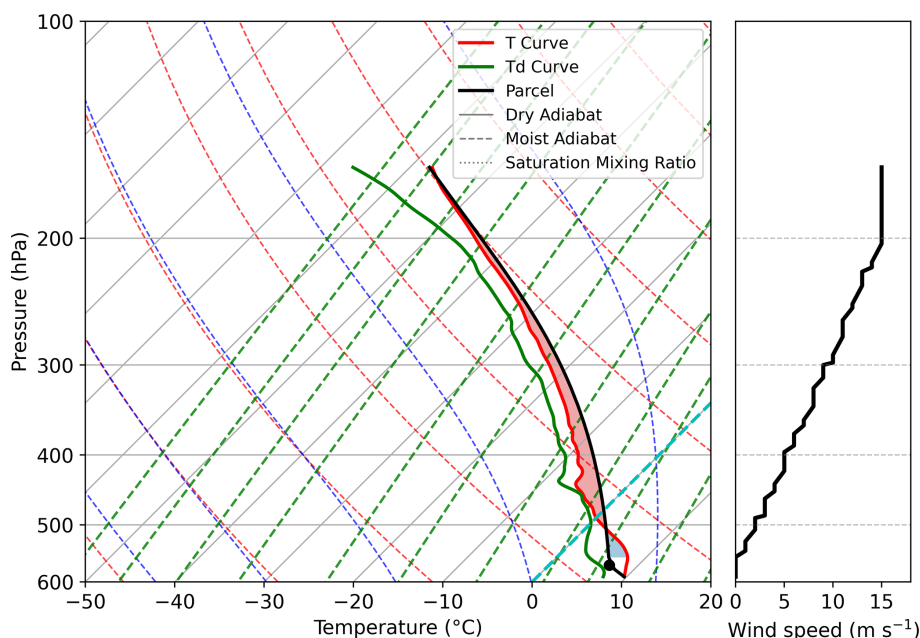
Figure 3. Skew T-lnp diagram illustrating the thermodynamic profile used to initialize all simulations.
