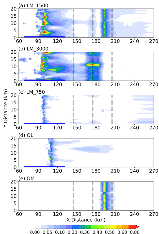
Figure 5. (a) Time-mean precipitation rate ( \text{mm h}^{-1} ) averaged over the 7–20 h period in LM_1500 (a) LM_1500, (b) LM_3000, (c) LM_750, (d) OL, and (e) OM. The thick blue line indicates the lake area ( x = 70–130 \text{ km} ), and the gray dashed lines mark the windward foothill ( x = 145 \text{ km} ), mountain summit ( x = 175 \text{ km} ), and leeward foothill ( x = 205 \text{ km} ).
