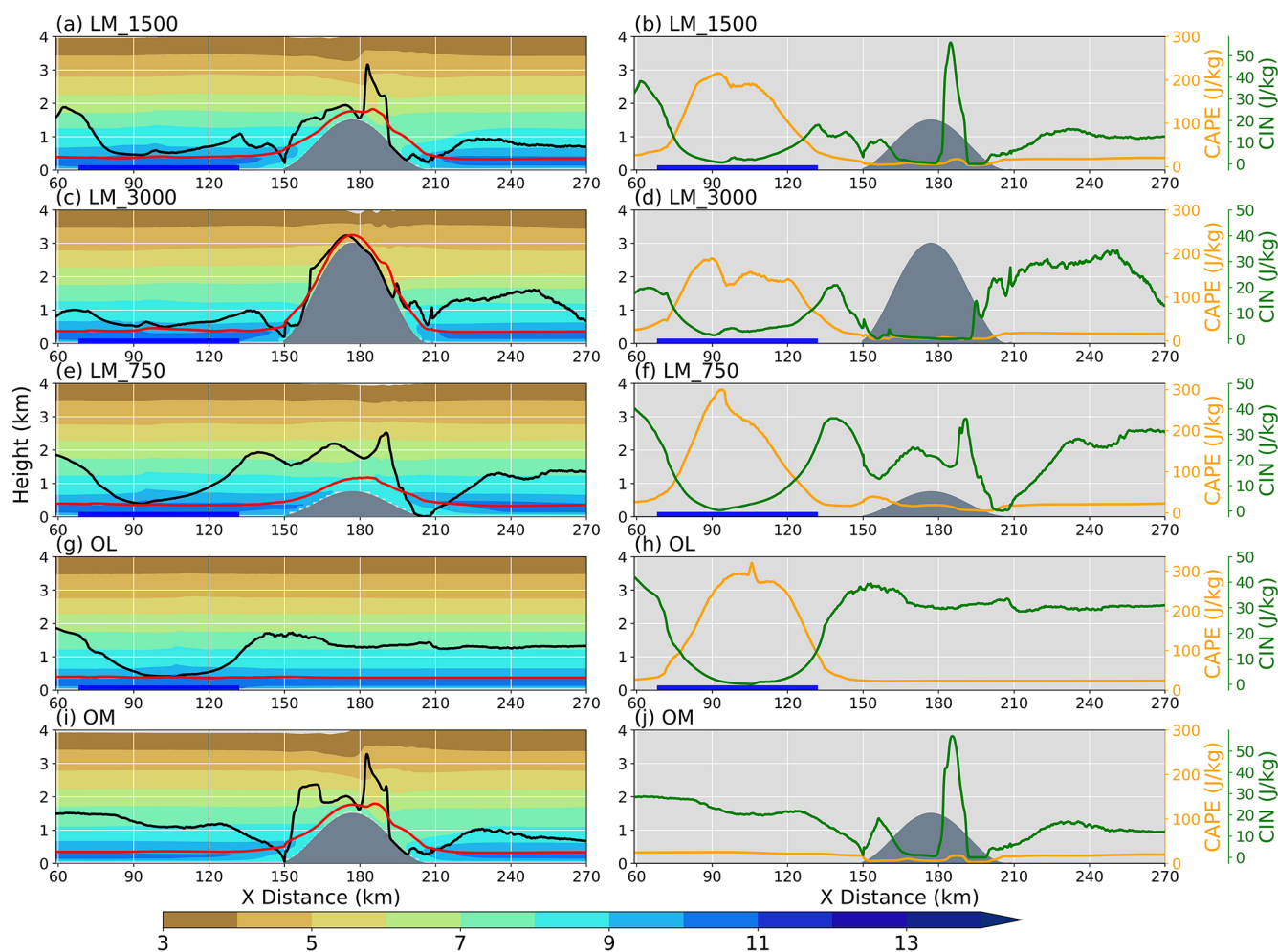
Figure 6. (a, b) Vertical cross sections of the 7–20 h time-mean, y-averaged water vapor mixing ratio (shading, \text{g kg}^{-1} ) in the LM_1500. The left panels (a) show the lifted condensation level (LCL; red lines) and the level of free convection (LFC; black lines). The right panels (b) show the surface-based convective available potential energy (CAPE; orange lines, right axis) and convective inhibition (CIN; green lines, left axis) along the cross section. (c–d, e–f, g–h, i–j) As in (a, b), but for the LM_3000, LM_750, OL, and OM, respectively. The thick blue line represents the lake surface, and the gray shading represents the terrain height (m).
