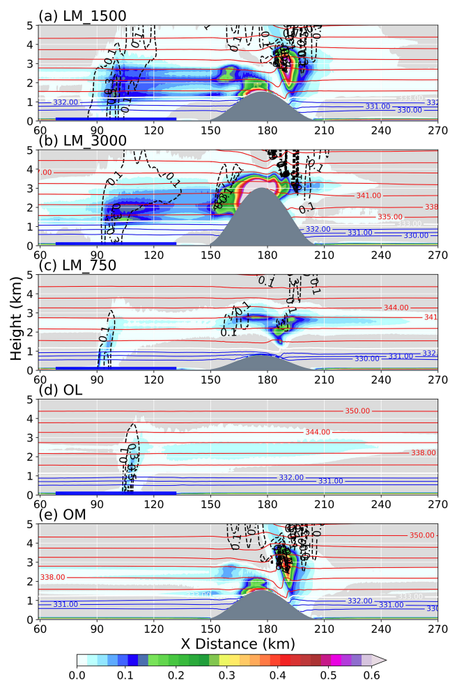
Figure 7. (a) Vertical cross sections of the 7–20 h time-mean, y-averaged total hydrometeor mixing ratio (shading, \text{g kg}^{-1} ) in the LM_1500. The potential temperature (blue-to-red contour lines, K) and vertical velocity (black dashed contour lines, only plotted positive values, \text{m s}^{-1} ). The vertical velocity field is smoothed with a 20 \times 20 -point uniform filter. Panel (b–e), same as panel (a), but for the LM_3000, LM_750, OL, and OM, respectively. The thick blue line represents the lake surface, and the gray shading represents the terrain height (m).
