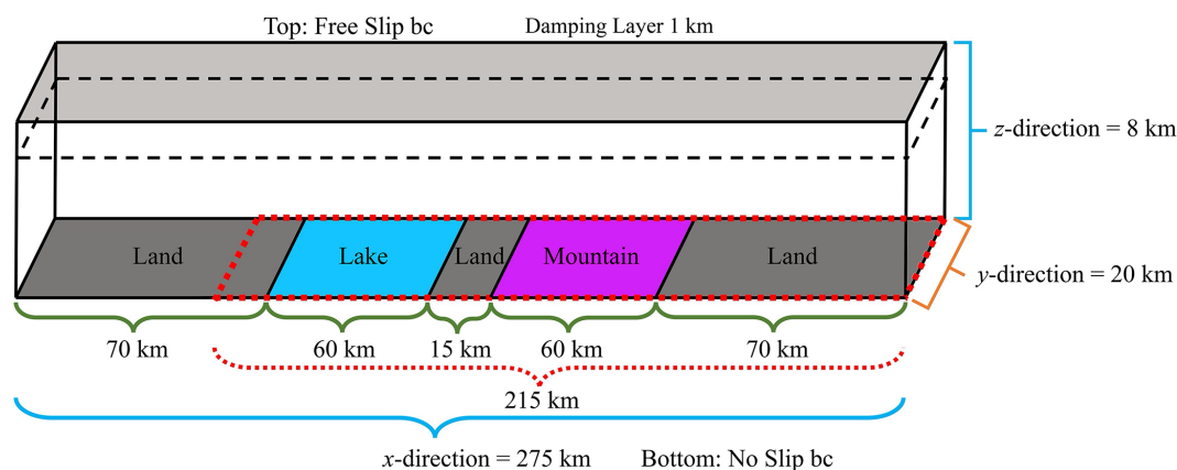
Figure 2. Domain configuration sketches of heterogeneous underlying surfaces. The blue and purple domains represent the lake and mountain, respectively. The areas in red dash boxes are analyzed areas.
