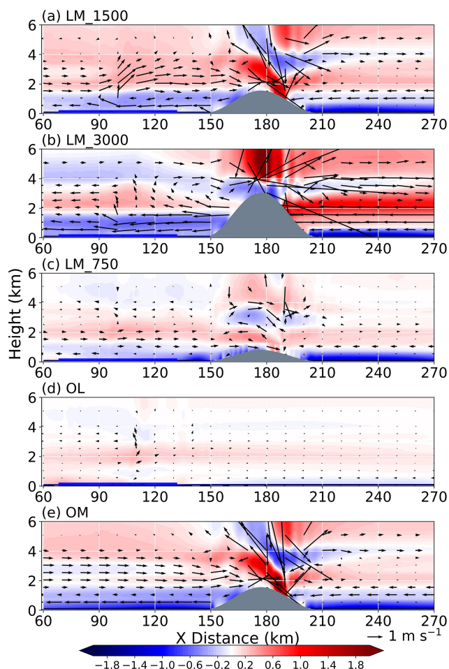
Figure 10. (a) Vertical cross sections of the 7–20 h time-mean, y-averaged perturbation potential temperature (shading, \theta' , K) in the LM_1500. The cross-section-parallel wind vectors composed by the perturbation zonal wind ( u' ) and vertical velocity ( w ). The reference arrow indicates a wind speed of 1 \text{ m s}^{-1} . The wind-vector field is smoothed with a 20 \times 20 -point uniform filter. (b–e) As in (a), but for the LM_3000, LM_750, OL, and OM experiments, respectively. The thick blue line represents the lake surface, and the gray shading represents the terrain height (m).
