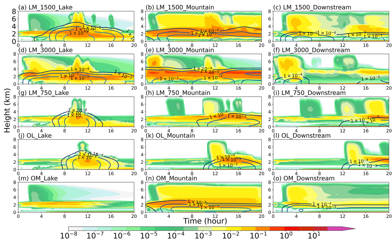
Figure 8. Temporal evolution of cloud condensate mixing ratios averaged in y -direction. The vertical axis denotes height above local ground level (km a.g.l.). Colored shading shows the total cloud condensate q_{hc} = q_c + q_i + q_s + q_g (including cloud water, cloud ice, snow, and graupel; \text{g kg}^{-1} ), and contour lines denote the rainwater mixing ratio q_r ( \text{g kg}^{-1} ), both averaged over the (left) lake, (middle) mountain, and (right) downstream subregions. Panels (a–c) correspond to LM_1500, (d–f) to LM_3000, (g–i) to LM_750, (j–l) to OL, and (m–o) to OM.
