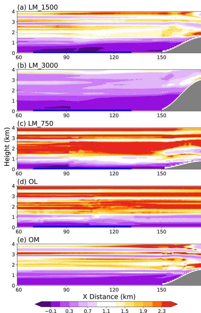
Figure 11. (a) Vertical cross sections of the 7–20 h time-mean, y-averaged moist flow-stability index in the LM_1500. (b–e) as in (a), but for the LM_3000, LM_750, OL, and OM, respectively. The thick blue line represents the lake surface, and the gray shading represents the terrain height (m).
