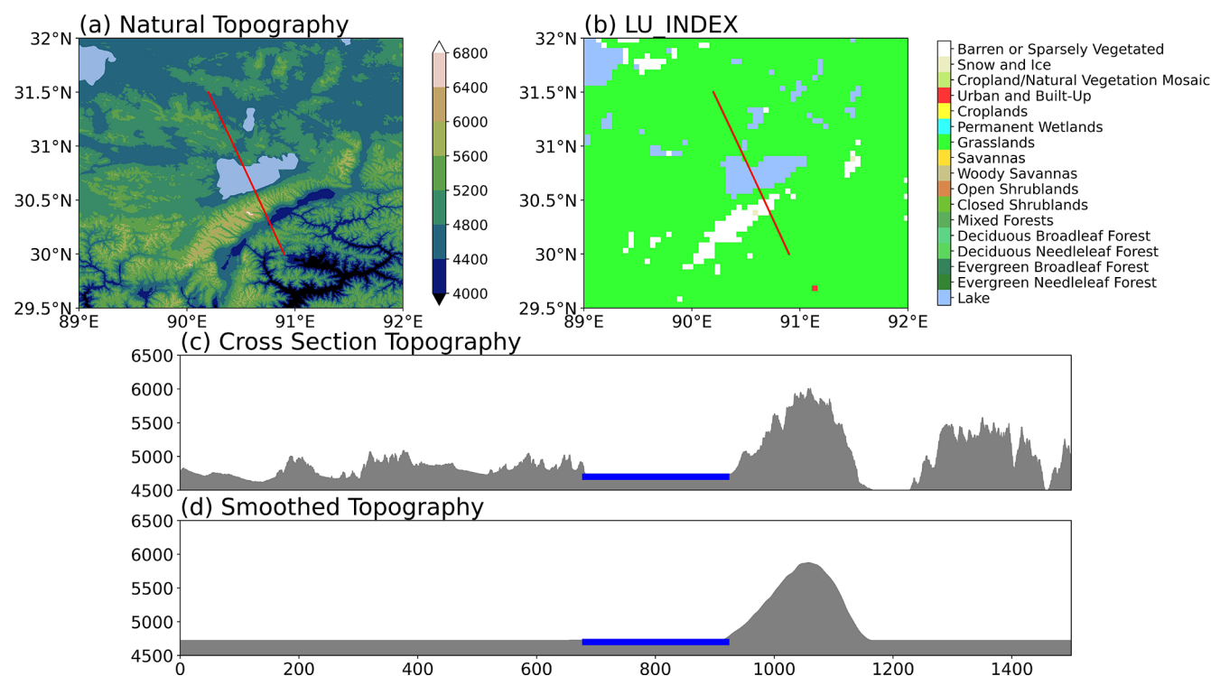
Figure 1. Configuration of the idealized cross-sectional simulations. The red transect line passes through Nam Co Lake and the Nyenchen Thanglha Mountains, (a) incorporating realistic topography from SRTM and (b) land cover from MCD12C1. (c) Cross-sectional topography is extracted along this line. (d) The smoothed version is used in the simulations to isolate thermal and dynamical responses associated with the typical lake-mountain configuration.
