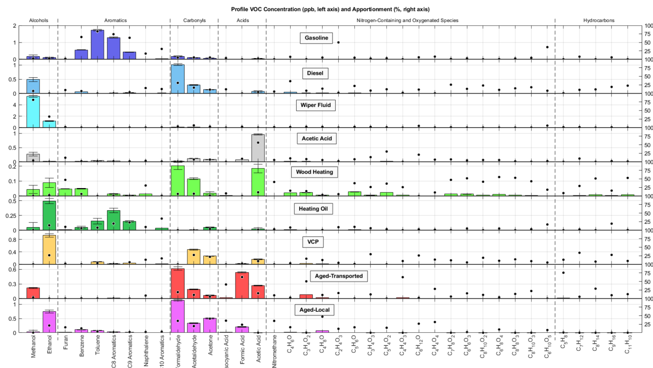
Figure 2. Mixing ratio (left y-axis, ppb) and percent apportionment (right y-axis) of VOCs assigned each factor. The x-label shows either the chemical name for species which are likely to be dominated by one isomer, or the chemical formula for species which are likely to have multiple isomers. The mixing ratio and percent for each species in each factor can be found in Tables S9 and S10, respectively.
