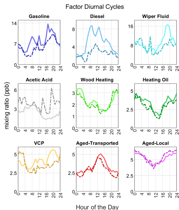
Figure 3. Mean diurnal cycles of all figures. The solid line is the weekday diurnal cycle (Monday through Friday), and the dashed line is the weekend diurnal cycle (Saturday and Sunday).
