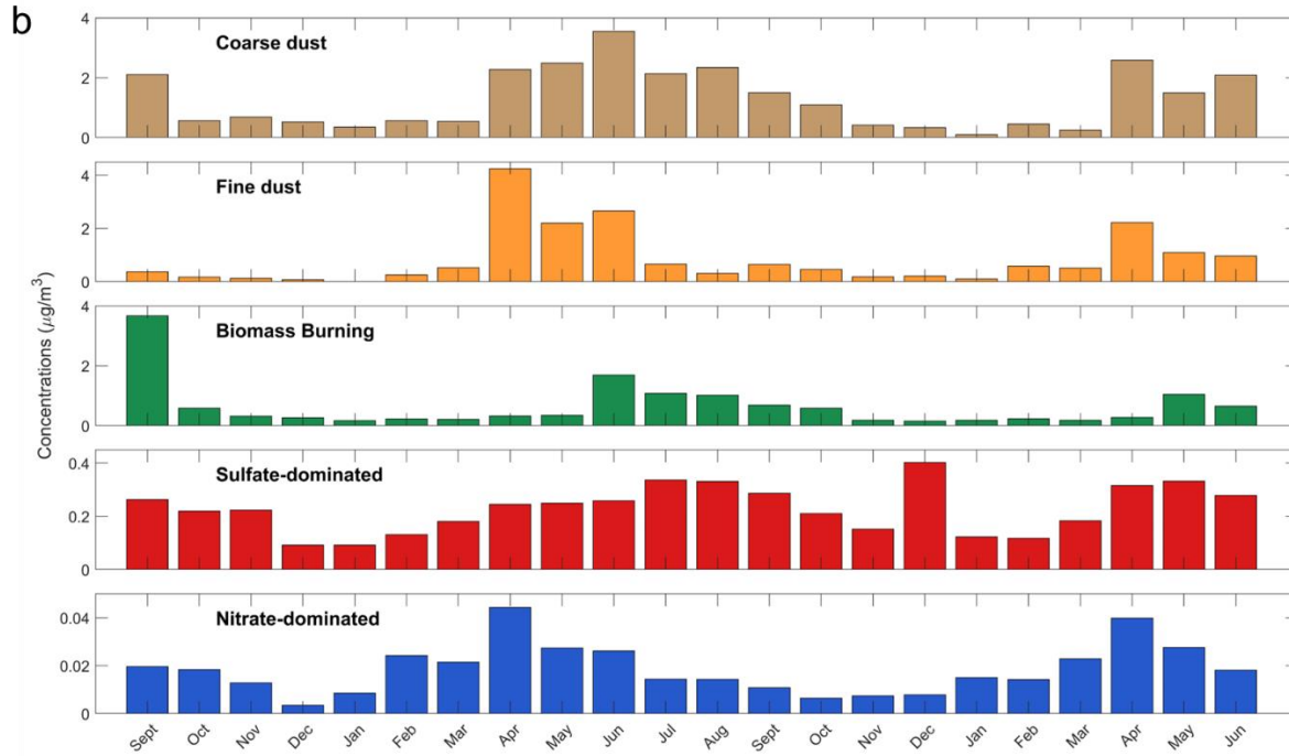
Figure S6. (a) Time series of mass concentrations ( \mu\text{g m}^{-3} ) attributed to the five factors during the period of the SAIL campaign (September 2021 to June 2023), and (b) their monthly mean concentrations.
