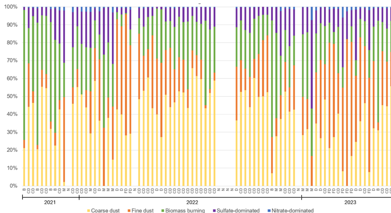
Figure S8. Proportions of source contributions for all samples. The label below each sample indicates its classification: CD (coarse dust), B (biomass burning), D(dust), FD (Fine dust), M (Mixed sources), and N (no source information).
