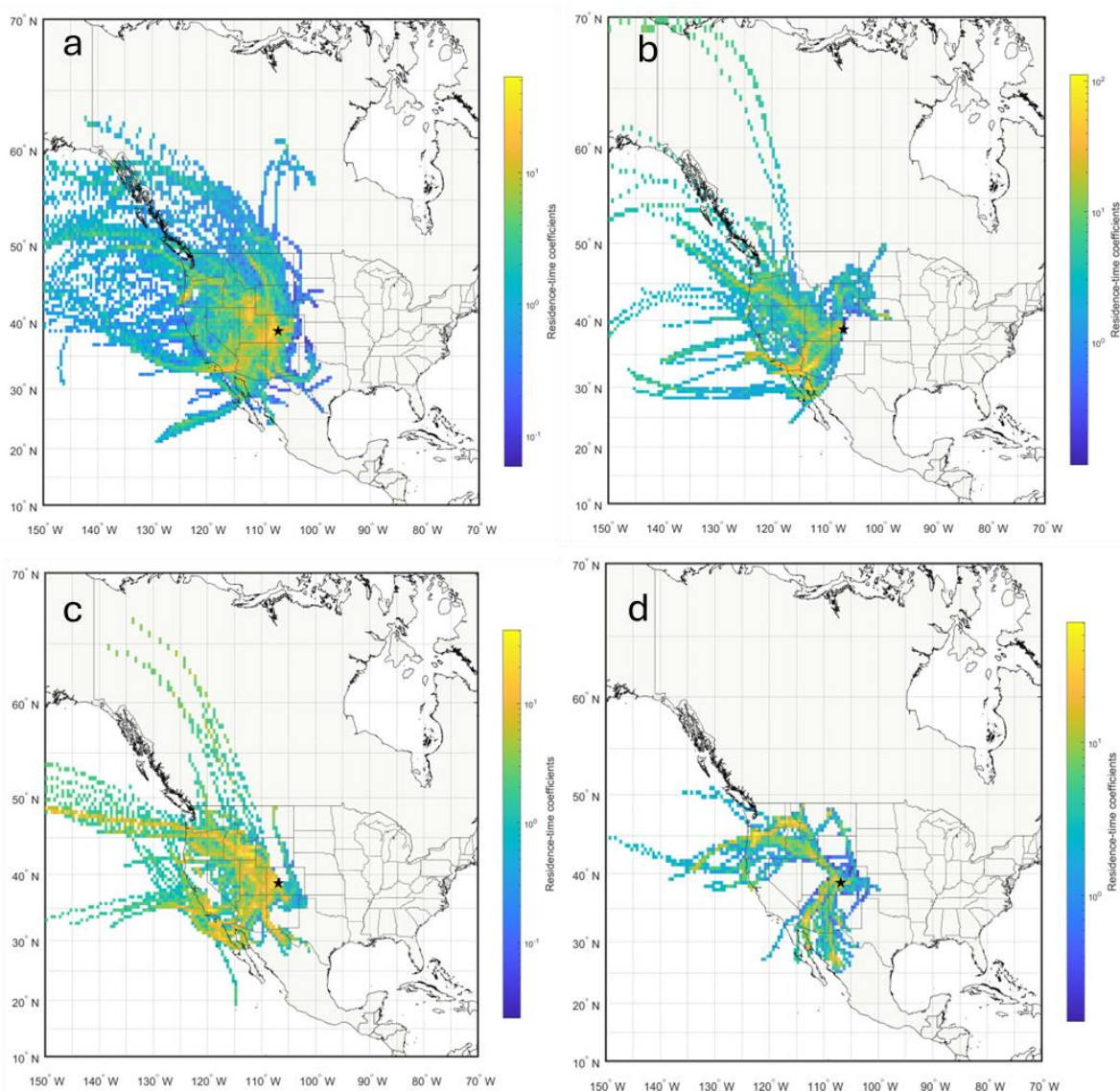
Figure S9. Residence-time weighted back trajectories for samples that were categorized as dominated by (a) coarse dust, (b) fine dust, (c) dust, and (d) biomass burning. The categorization was based on aerosol source contributions derived from the PMF analysis; details of the categorization method are provided in the Methods section. The black stars mark the SAIL sampling location.
