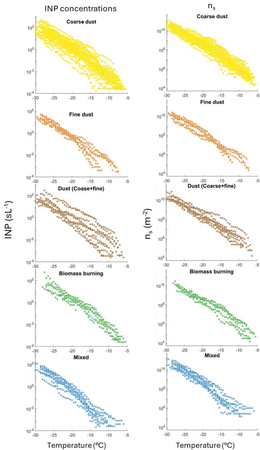
Figure S11. Total INP temperature spectra (sL -1 ) and IN active surface site density ( n_s , m -2 ) stratified by dominant aerosol source (coarse dust, dust, fine dust, biomass burning, and mixed). n_s is calculated based on the surface area of particles larger than 500 nm.
