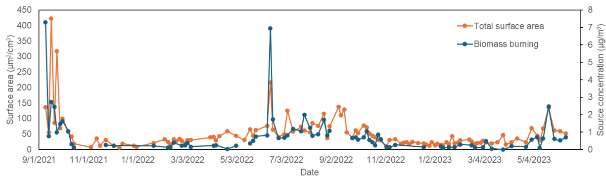
Figure S12. Relationships between biomass burning mass concentration ( \mu\text{g}/\text{m}^3 ) and total surface area concentrations ( \mu\text{m}^2/\text{cm}^3 ).
