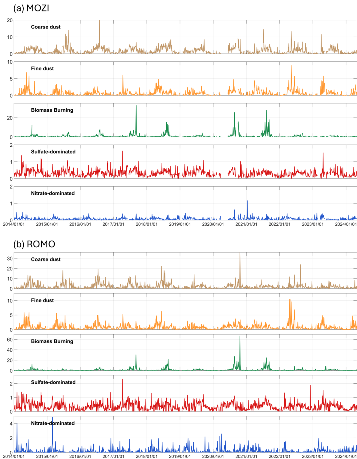
Figure S7. Time series of aerosol type concentrations ( \mu\text{g m}^{-3} ) for the five-factor solution from the PMF analysis of data from the IMPROVE site at (a) Mount Zirkel Wilderness (MOZI) and (b) Rocky Mountain NP (ROMO).
