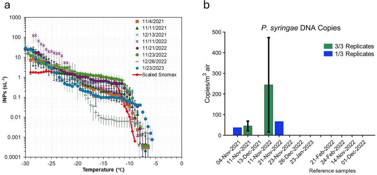
Figure S4. (a) INP temperature spectra for wintertime samples with a distinct shape similar to that of Snomax. (b) P. syringae DNA copy numbers in these samples and in reference samples presumed not affected by Snomax, according to inspection of their INP spectra.
