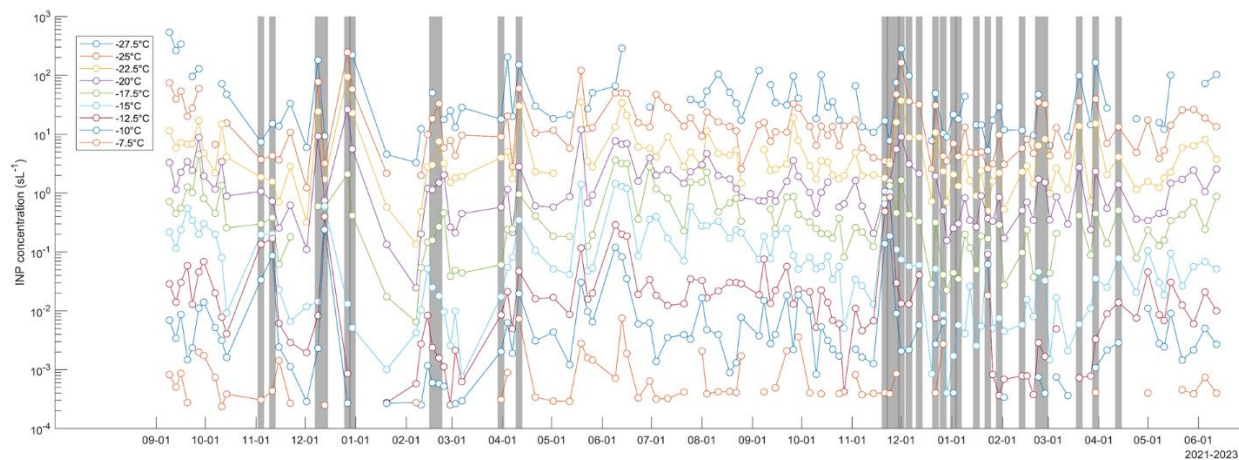
Figure S3. INP concentrations ( \text{sL}^{-1} ) at temperatures from -7.5^\circ\text{C} to -27.5^\circ\text{C} (interval of 2.5^\circ\text{C} ) for all analyzed samples during SAIL campaign. The grey shadows show samples collected during cloud seeding and affected by snowmaking activities.
