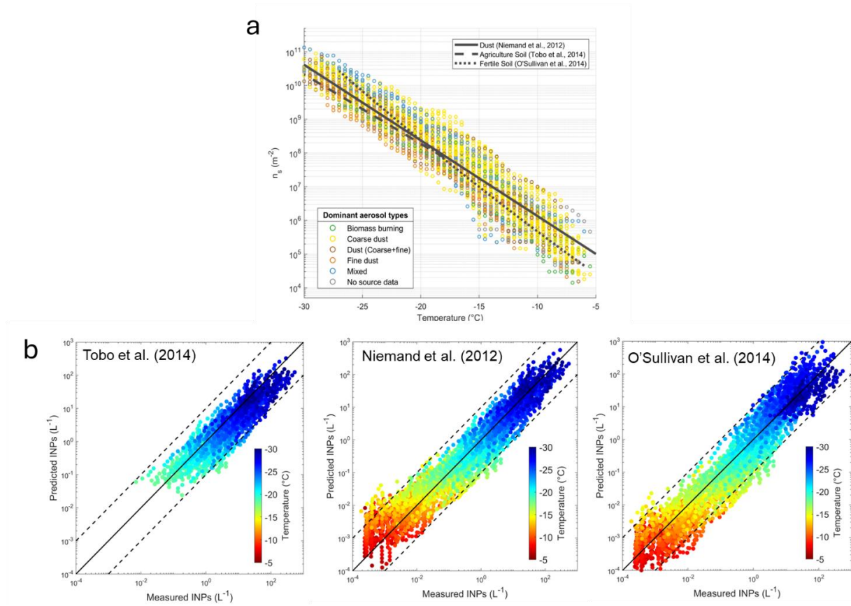
Figure S14. (a) IN active surface site density ( n_s , \text{m}^{-2} ) calculated based on the surface area of particles larger than 500 nm, compared with those derived from agricultural soil (Tobo et al., 2014), dust (Niemand et al., 2012), and fertile soil (O'Sullivan et al., 2014). (b) Estimated SAIL INP concentrations using parameterizations from Tobo et al. (2014), Niemand et al. (2012), and O'Sullivan et al. (2014) and surface area of particles larger than 500 nm, compared with SAIL observations.
